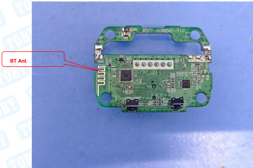
Photo 16 Appearance of PCB
