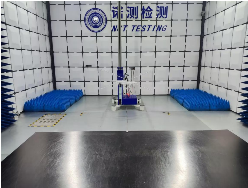
Setup Photo FCC ID: 2BBN9-002
