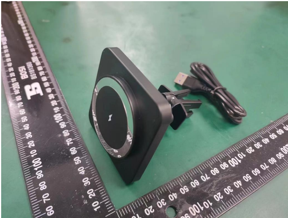
External Photo FCC ID: 2BBMP-CW601
