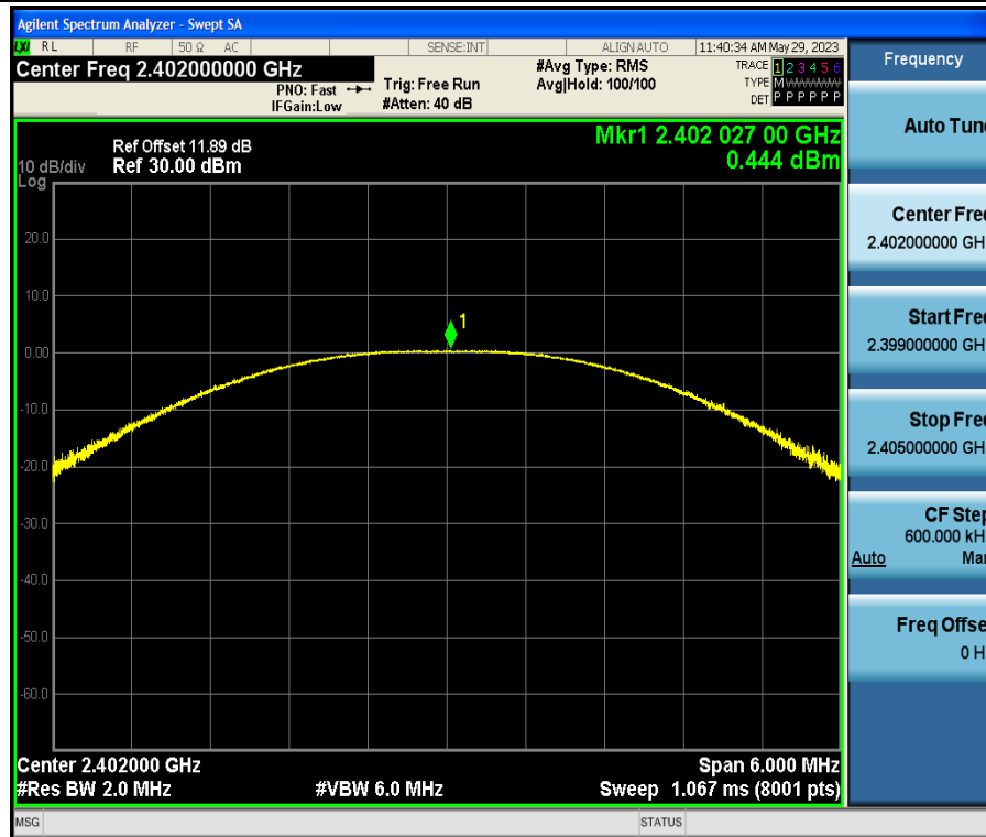
BLE_1M-Ant1-2402
