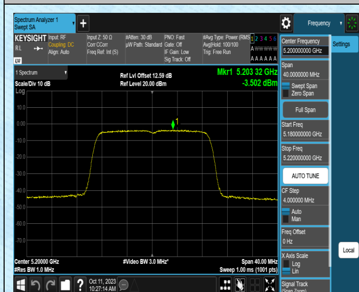
11AC20MIMO-Ant1-5200-PASS
