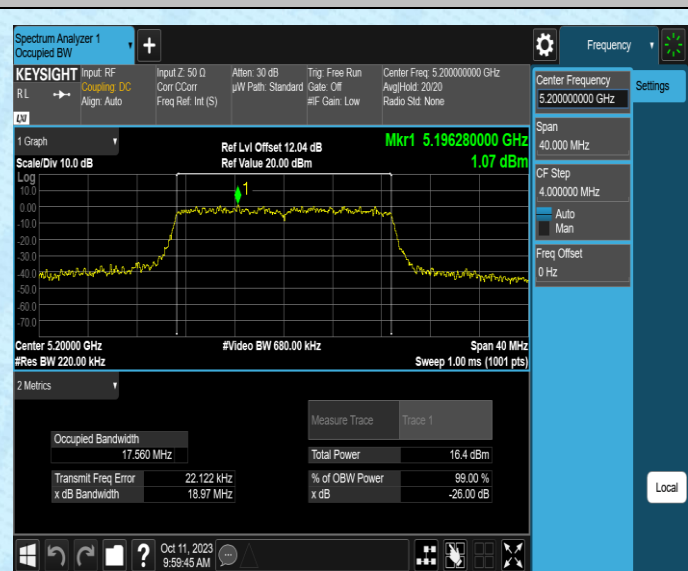
11N20SISO-Ant2-5200
