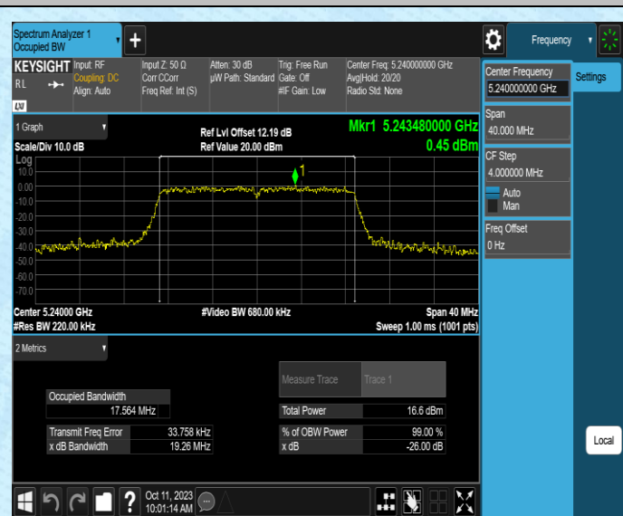
11N20SISO-Ant2-5240
