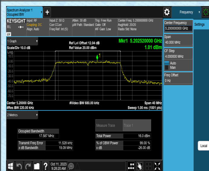
11AC20SISO-Ant1-5200
