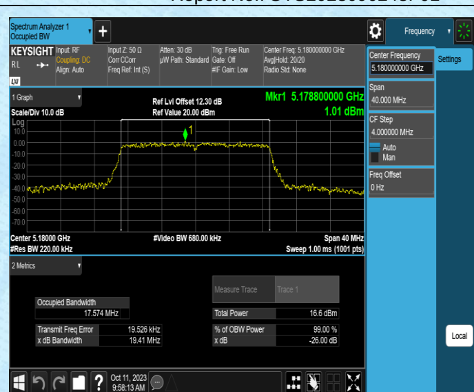
11N20SISO-Ant2-5180
