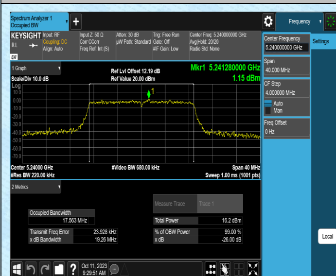
11AC20SISO-Ant1-5240
