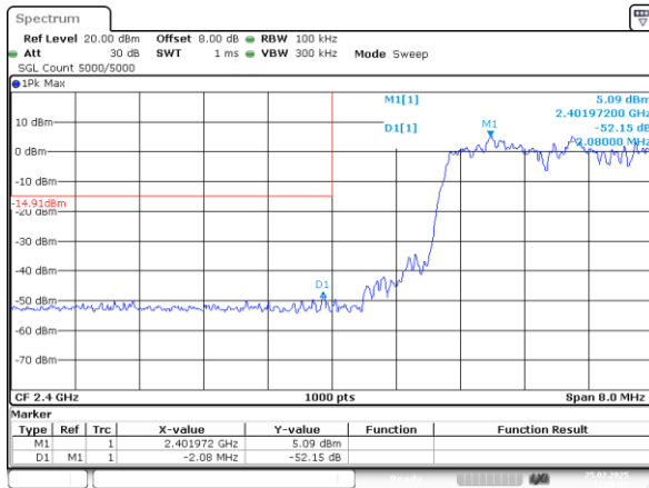
2DH1_Hopping_Lower 52.15dB
