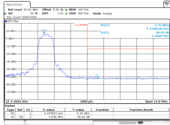
3DH1_High 56.65dB
