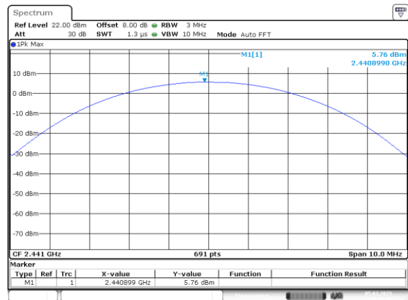
DH1_Middle 5.76dBm
