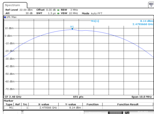
2DH1_High 8.14dBm
