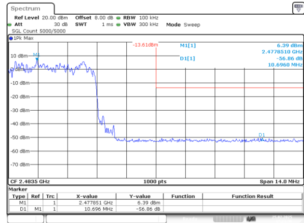
2DH1_Hopping_Upper 56.86dB
