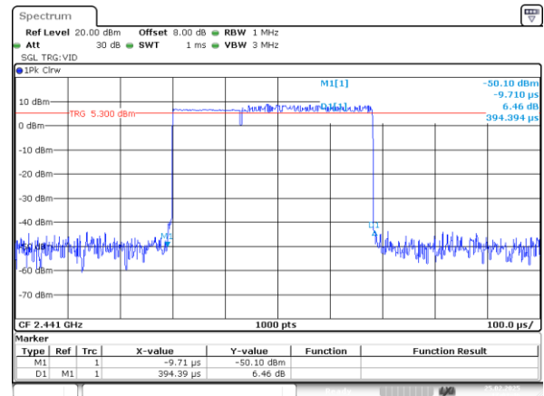
2DH1_Hopping 0.394ms
