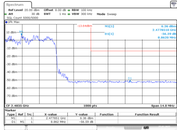
3DH1_Hopping_Upper 56.59dB
