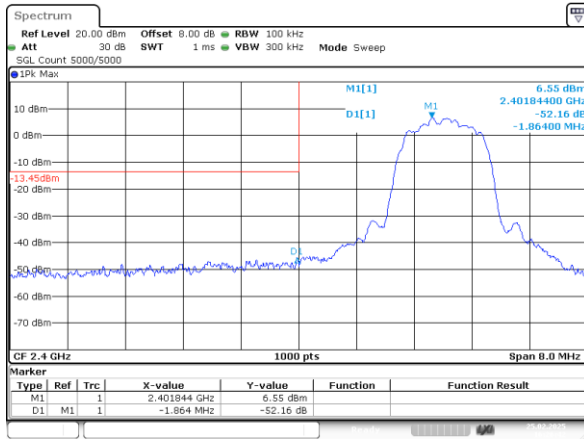
3DH1_Low 52.16dB
