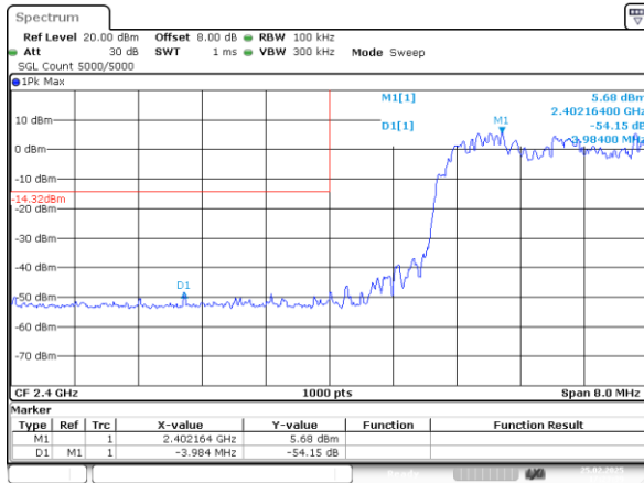
3DH1_Hopping_Lower 54.15dB
