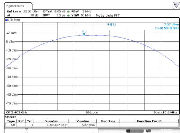
2DH1_Low 7.37dBm
