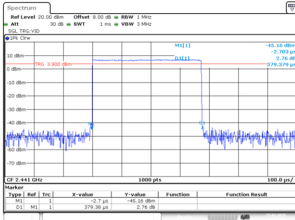
DH1_Hopping 0.379ms
