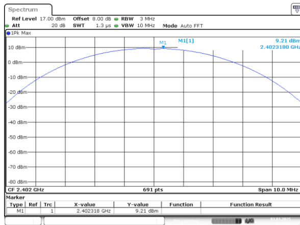
3DH1_Low 9.21dBm
