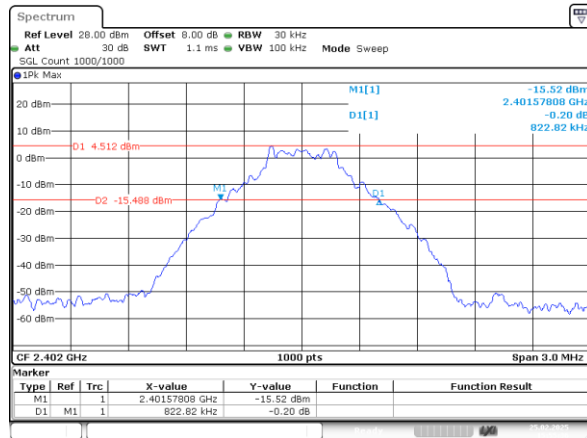
DH1_Low 0.823MHz
