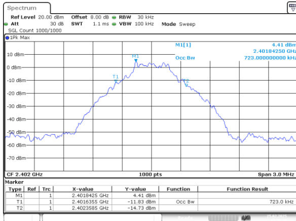
DH1_Low 0.723MHz
