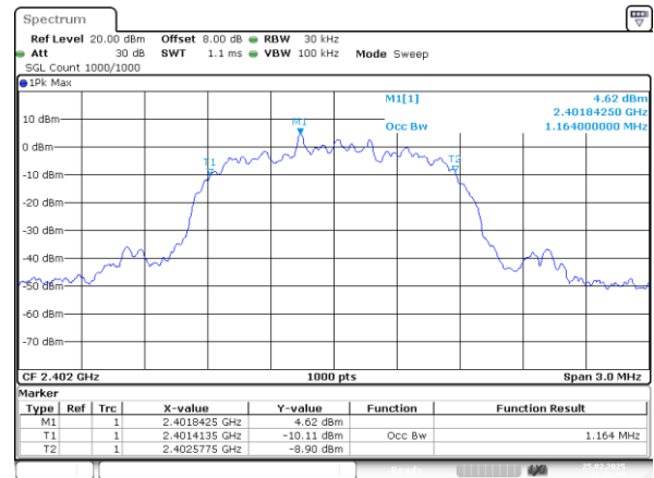
2DH1_Low 1.164MHz
