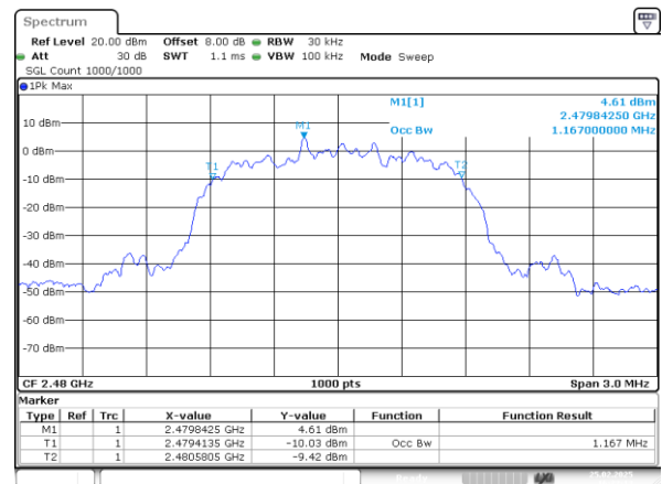
2DH1_High 1.167MHz
