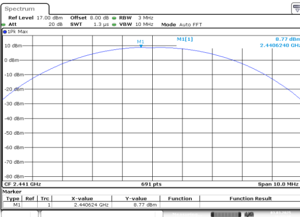
2DH1_Middle 8.77dBm
