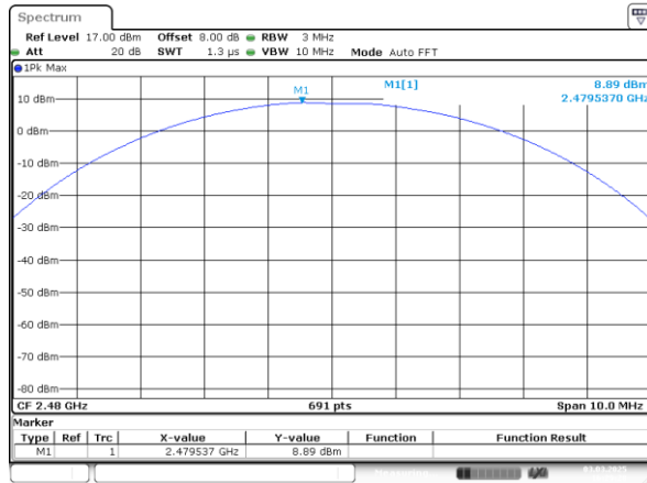
3DH1_High 8.89dBm
