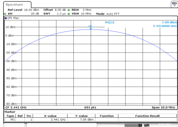
DH1_Middle 7.09dBm
