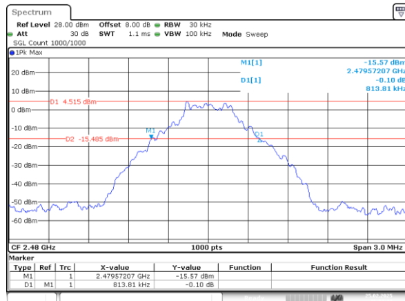
DH1_High 0.814MHz
