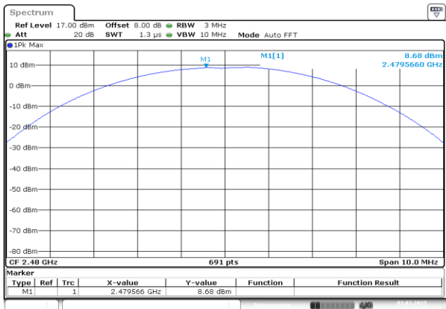
2DH1_High 8.68dBm
