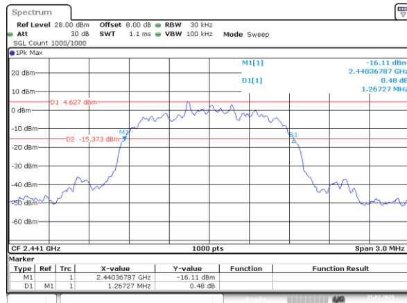
2DH1_Middle 1.267MHz
