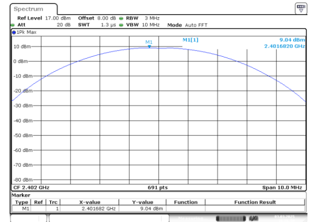
2DH1_Low 9.04dBm
