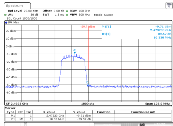
802.11n20_2472MHz_Chain 0
