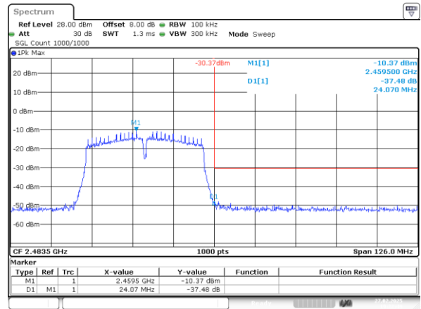
802.11n40_2462MHz_Chain 0
