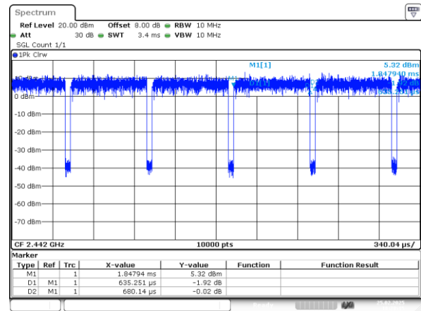
802.11n40_2442MHz_Chain 0
