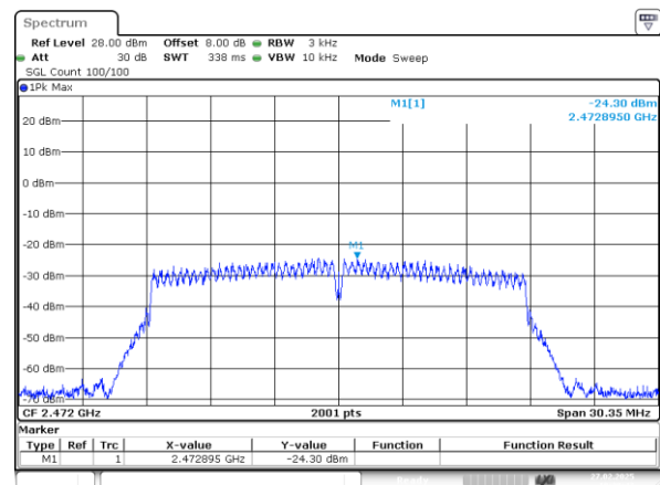
802.11n20_2472MHz_Chain 1
