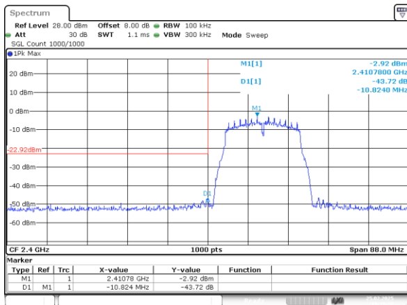
802.11g_2412MHz_Chain 1
