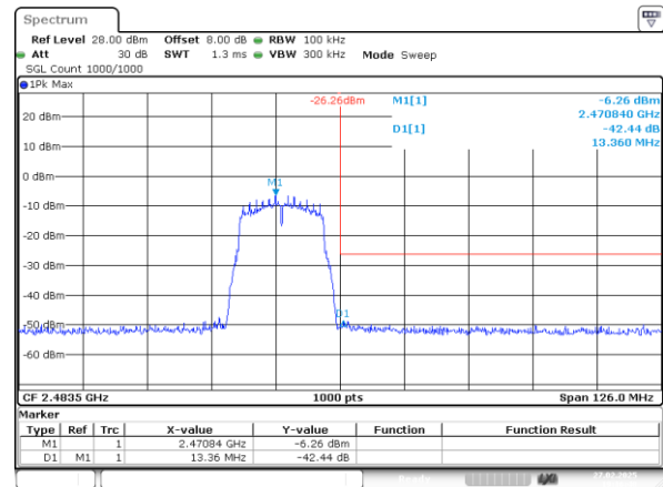
802.11g_2472MHz_Chain 0
