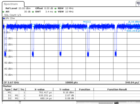
802.11n40_5670MHz_Chain 0
