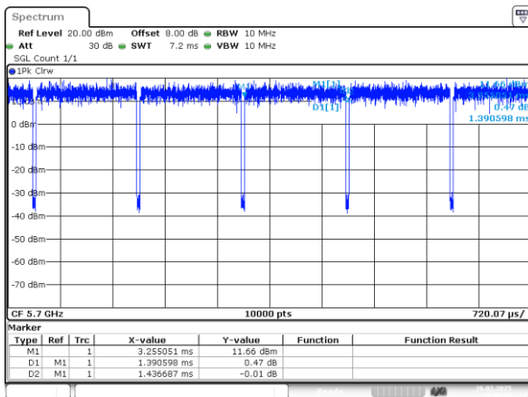
802.11a_5700MHz_Chain 0
