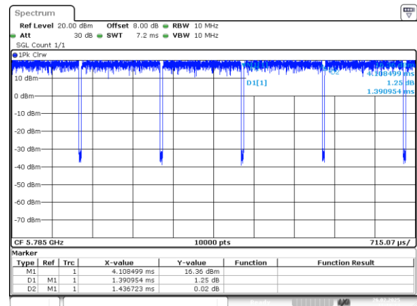
802.11a_5785MHz_Chain 0
