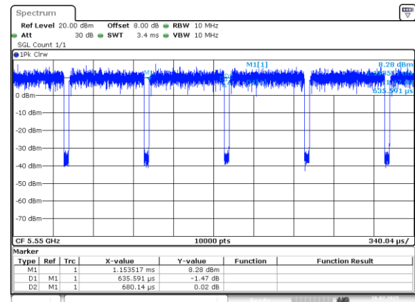
802.11n40_5550MHz_Chain 1
