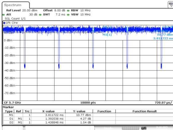
802.11a_5700MHz_Chain 1
