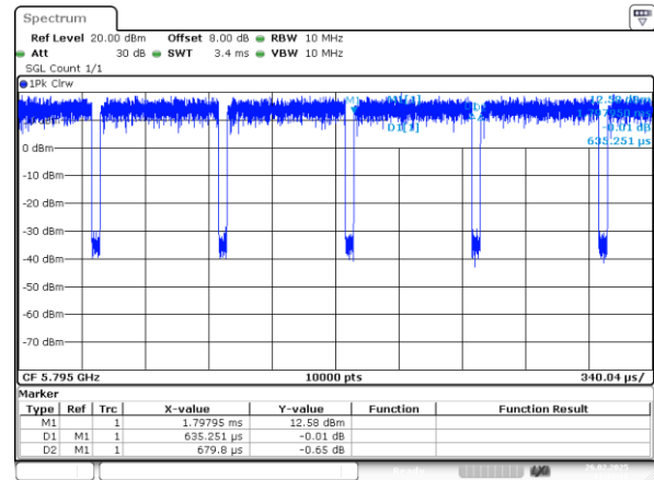
802.11n40_5795MHz_Chain 0
