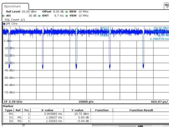
802.11n20_5280MHz_Chain 1
