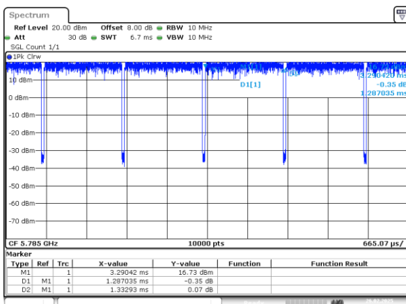
802.11n20_5785MHz_Chain 1
