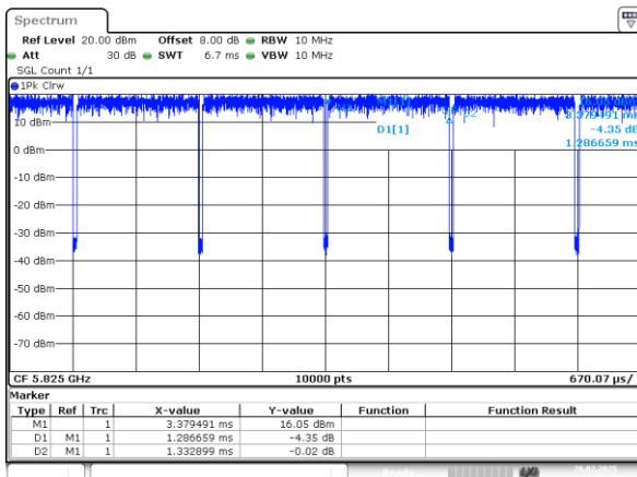
802.11n20_5825MHz_Chain 0
