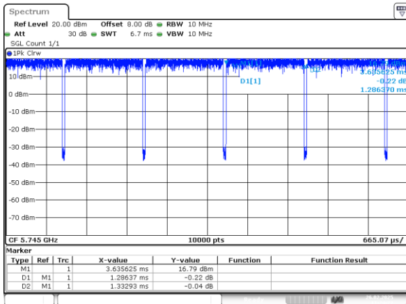
802.11n20_5745MHz_Chain 0
