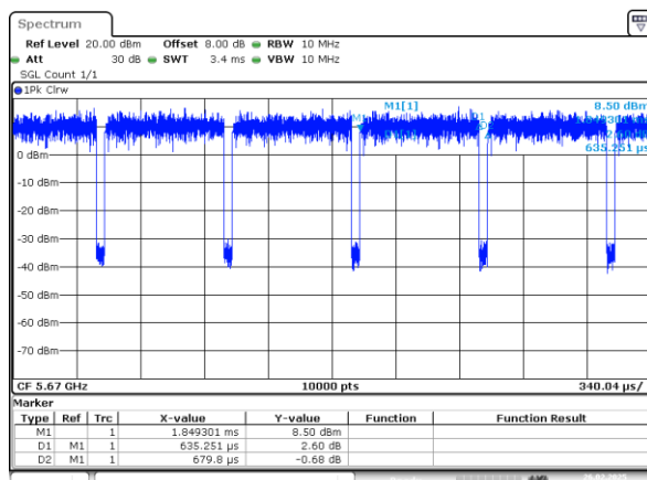
802.11n40_5670MHz_Chain 1
