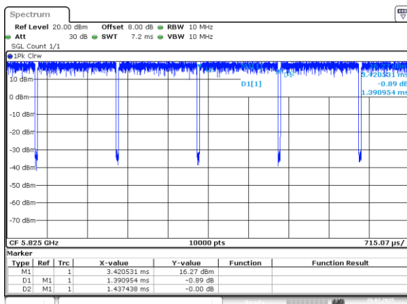
802.11a_5825MHz_Chain 0
