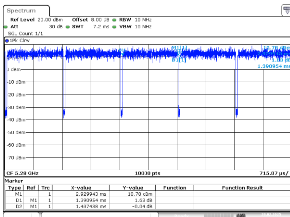
802.11a_5280MHz_Chain 1
