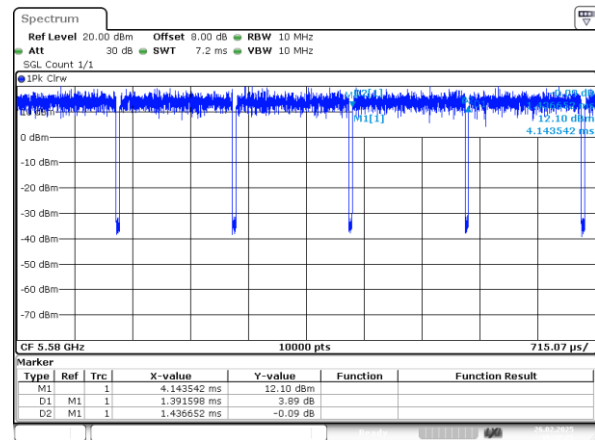
802.11a_5580MHz_Chain 0
