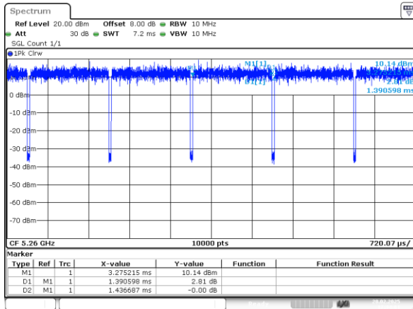
802.11a_5260MHz_Chain 0
