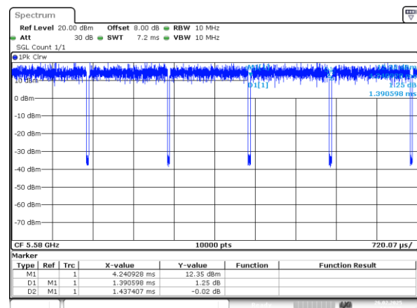
802.11a_5580MHz_Chain 1
