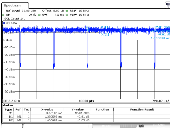
802.11a_5500MHz_Chain 0
