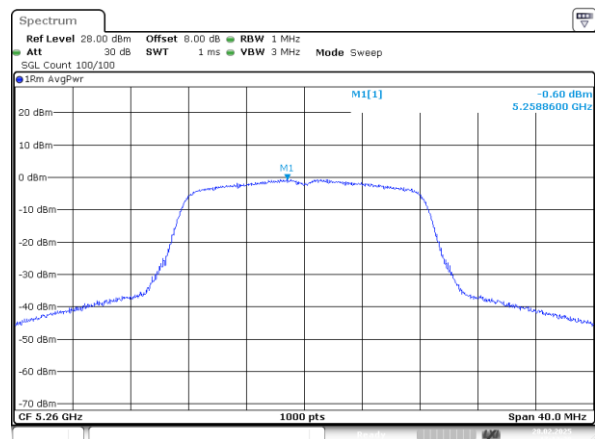
802.11a_5260MHz_Chain 1
