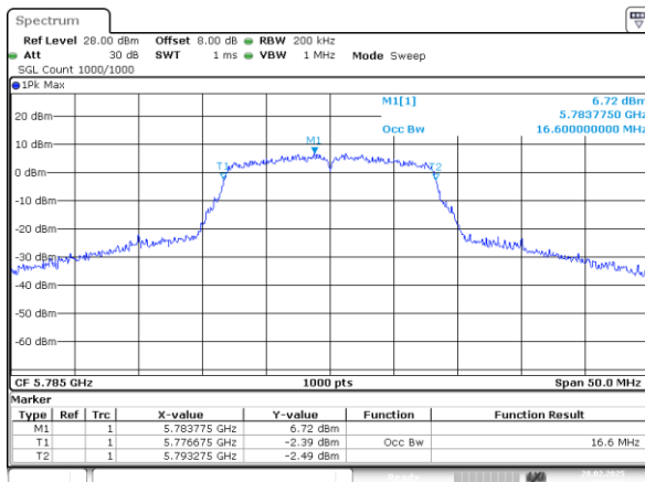
802.11a_5785MHz_Chain 1
