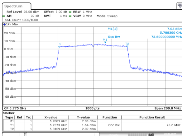
802.11ac80_5775MHz_Chain 0
