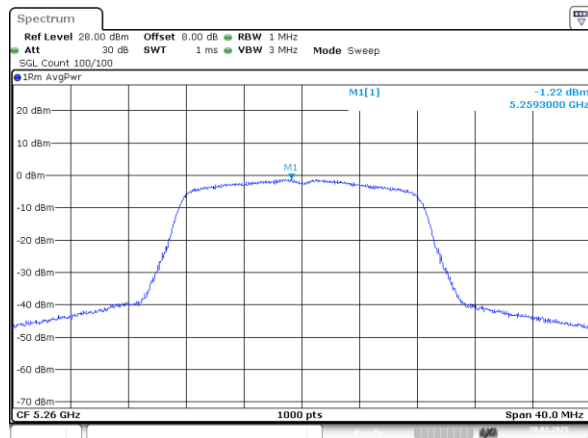
802.11a_5260MHz_Chain 0
