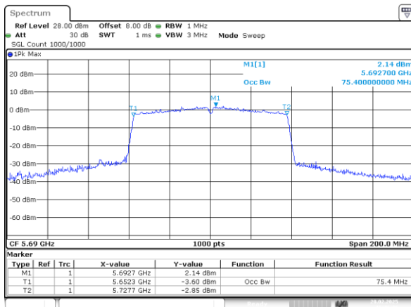
802.11ac80_5690MHz_Chain 0
