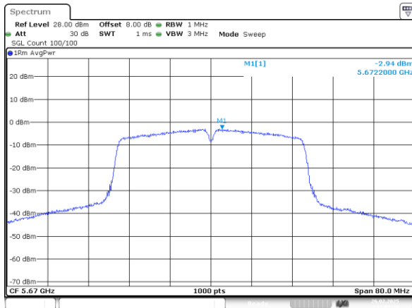
802.11n40_5670MHz_Chain 0
