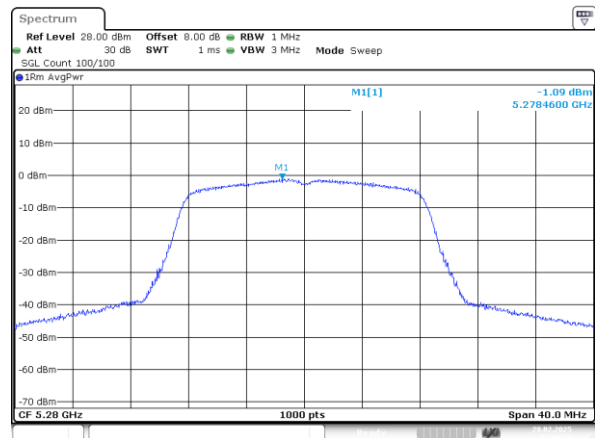
802.11a_5280MHz_Chain 0
