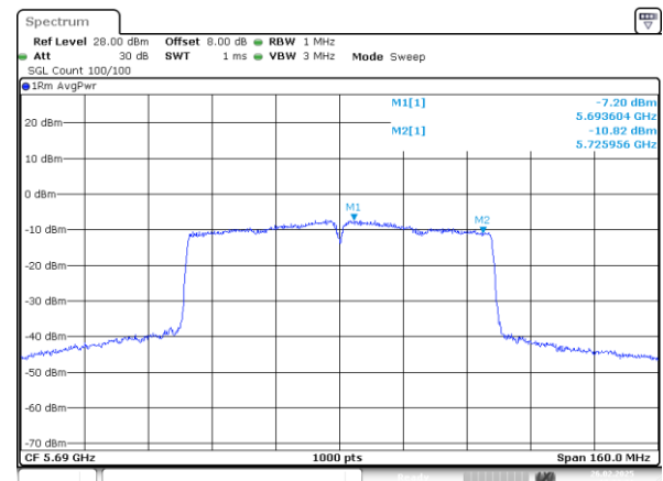
802.11ac80_5690MHz_Chain 1
