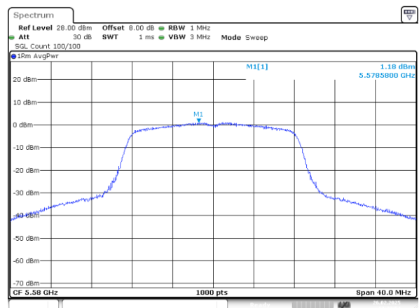
802.11a_5580MHz_Chain 1
