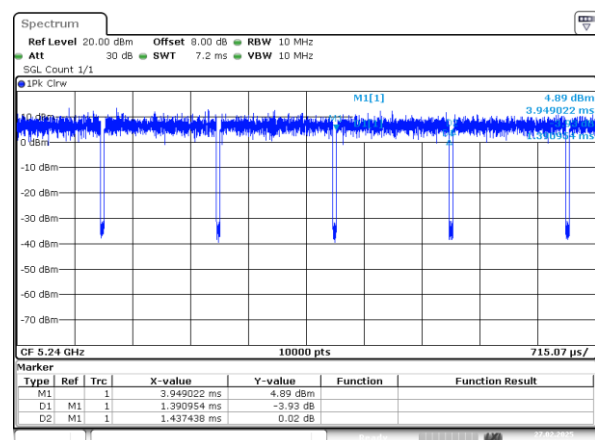
802.11a_5240MHz_Chain 1
