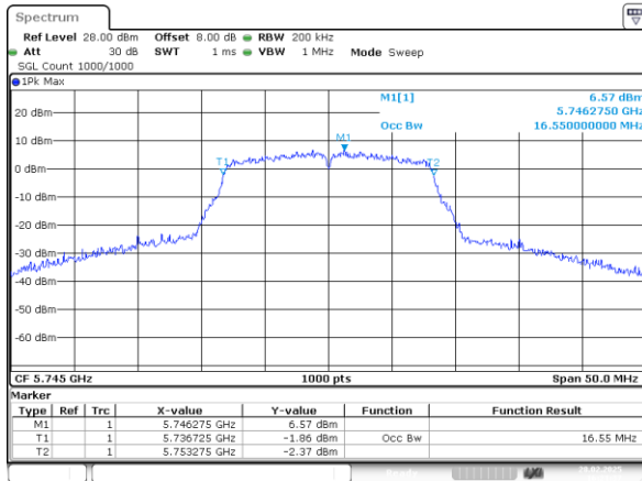
802.11a_5745MHz_Chain 0
