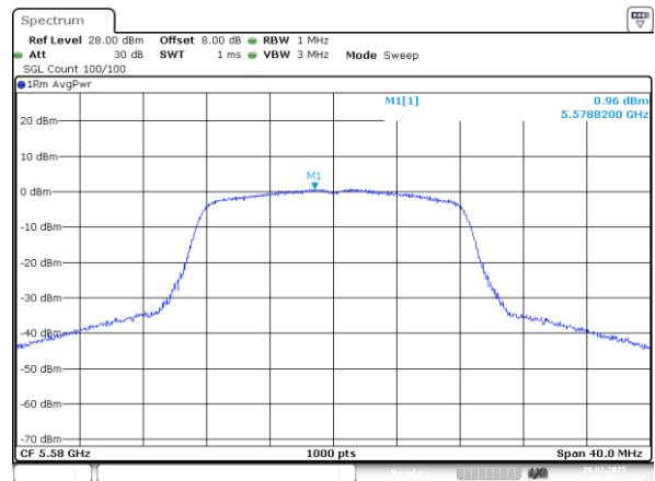
802.11a_5580MHz_Chain 0
