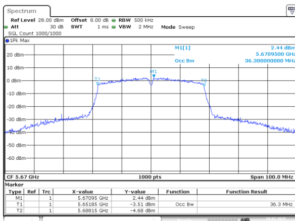
802.11n40_5670MHz_Chain 1
