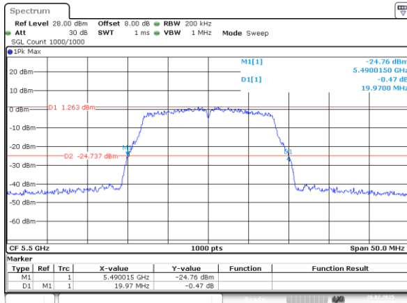
802.11a_5500MHz_Chain 0
