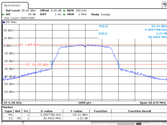
802.11a_5280MHz_Chain 1
