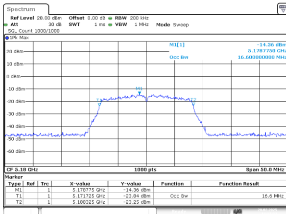
802.11a_5180MHz_Chain 0
