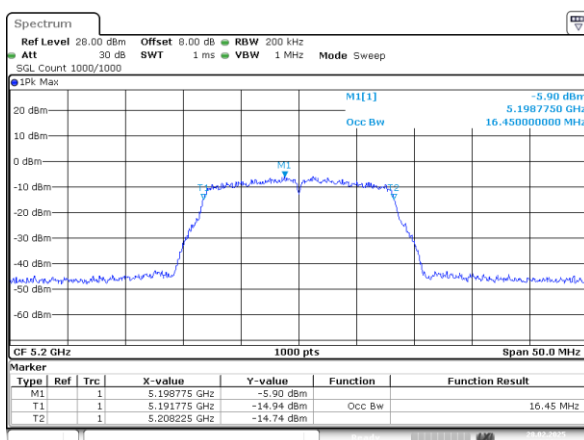
802.11a_5200MHz_Chain 1
