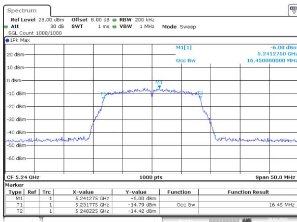
802.11a_5240MHz_Chain 0
