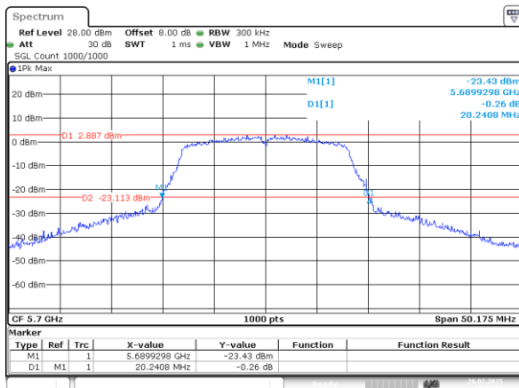
802.11a_5700MHz_Chain 0
