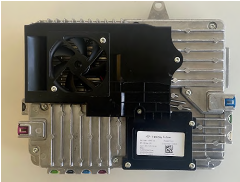
External Top View
