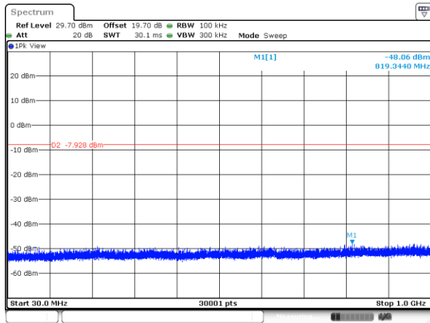
CSE Plot on Ch 78 between 30 MHz ~ 1 GHz
