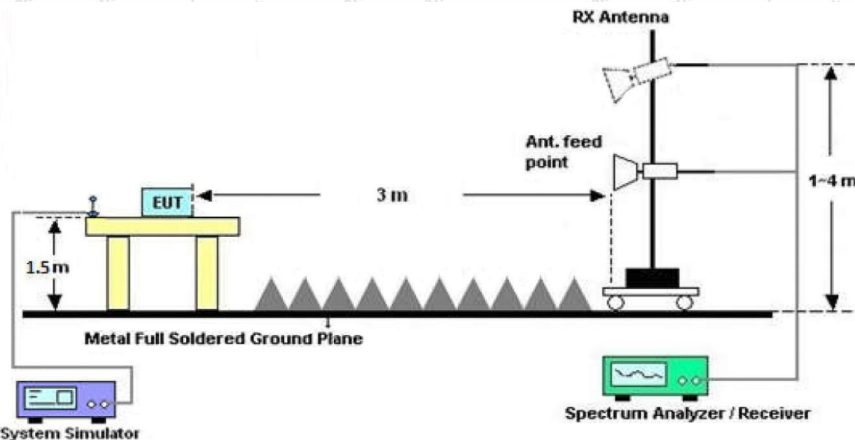
Figure 3. Above 1 GHz
