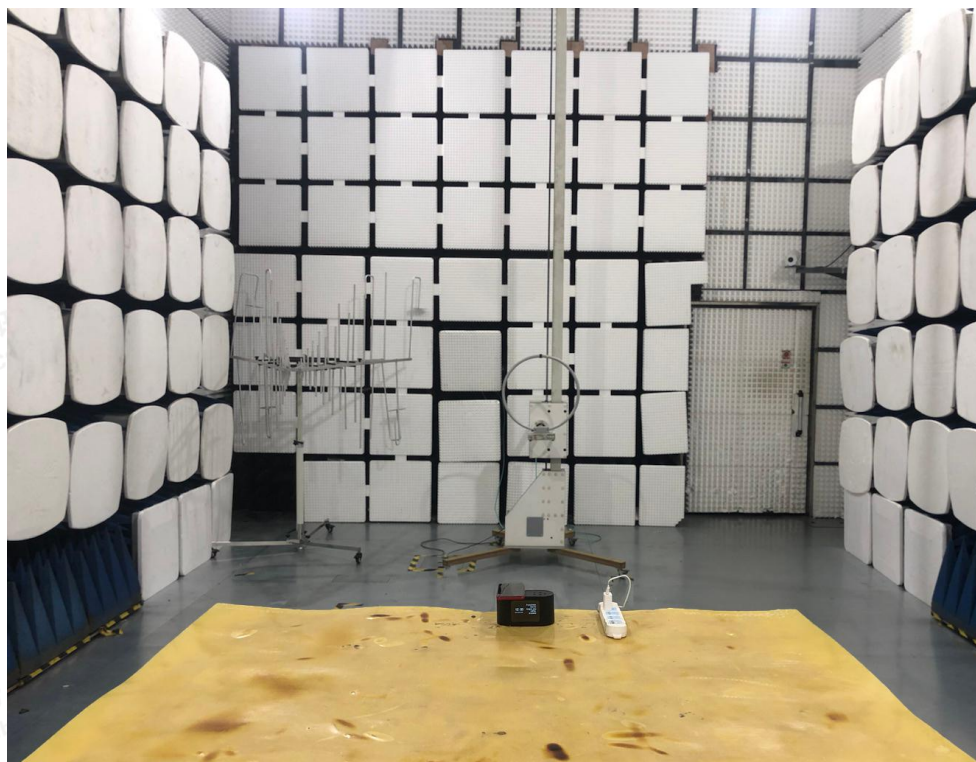
Radiated Emission below 30MHz-AC adapter charge mode
