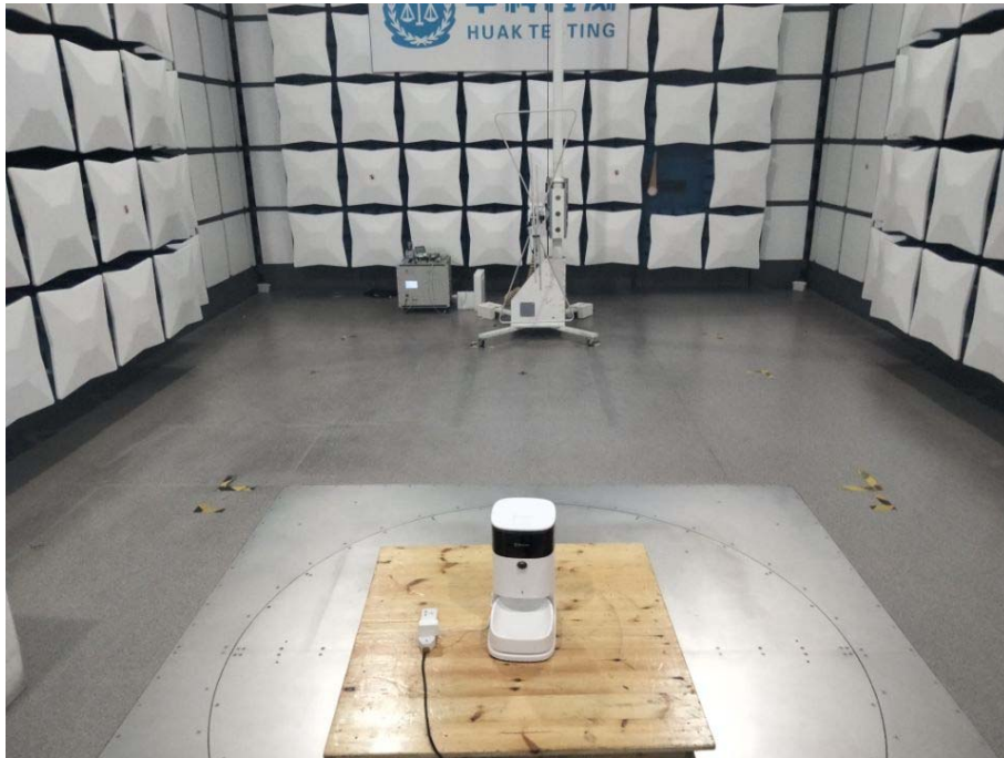
Model: PF2 Radiated Emissions
