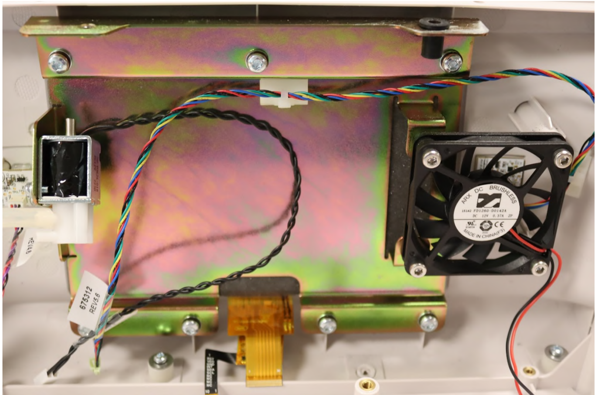
Boards removed (fan and chassis)
