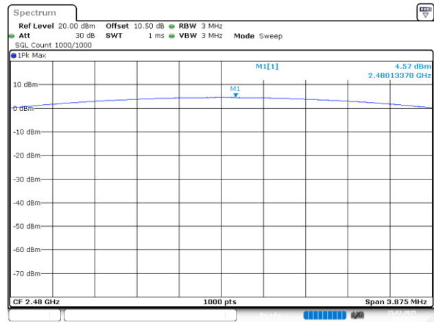
DH1_High
