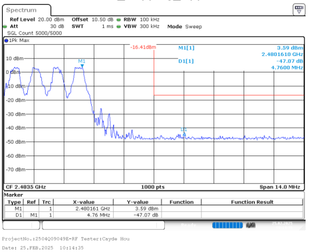
2DH1_High
