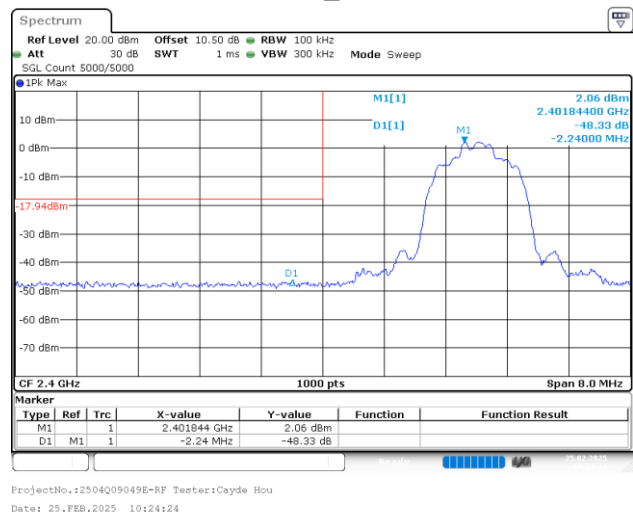
3DH1_Hopping_Lower
