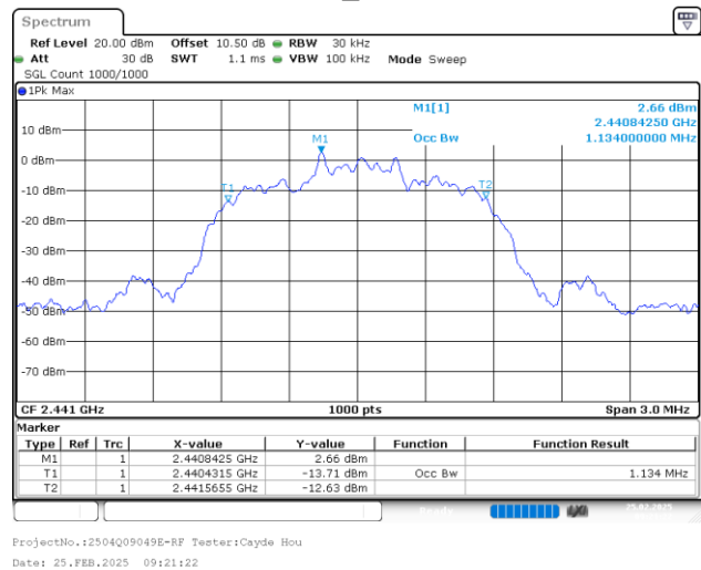
2DH1_Middle
