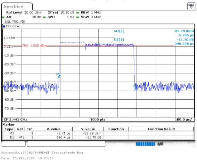
3DH1_Hopping
