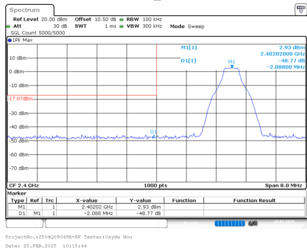
DH1_Hopping_Lower
