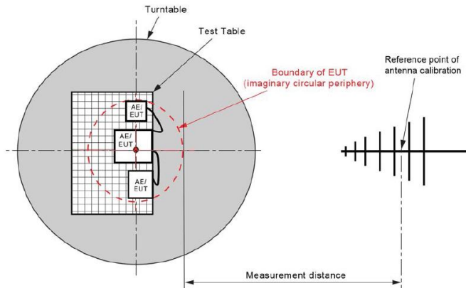
Figure C.1 – Measurement distance
