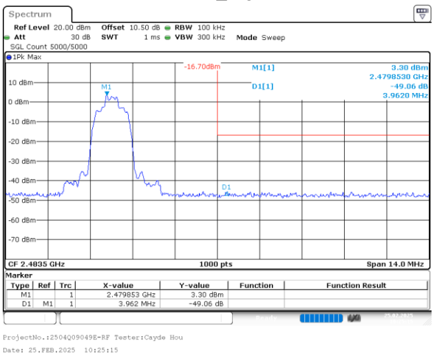
3DH1_Hopping_Upper
