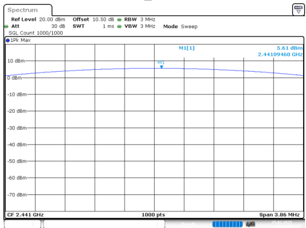
DH1_Middle
