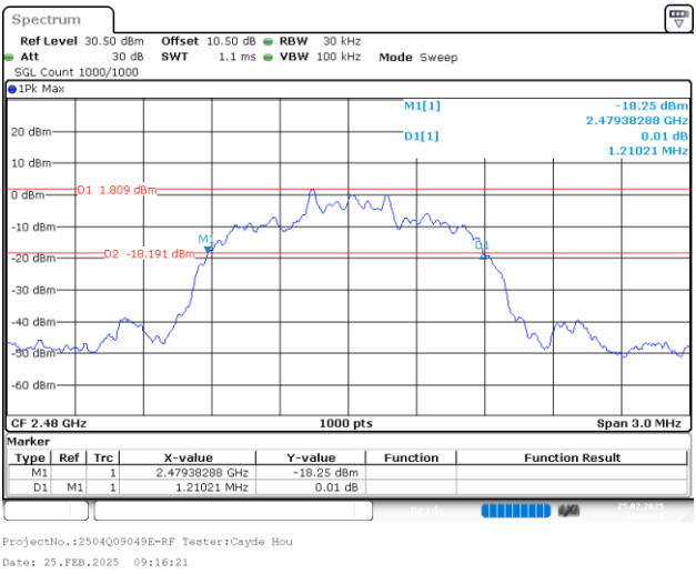
2DH1_High
