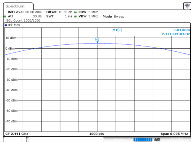
3DH1_Middle
