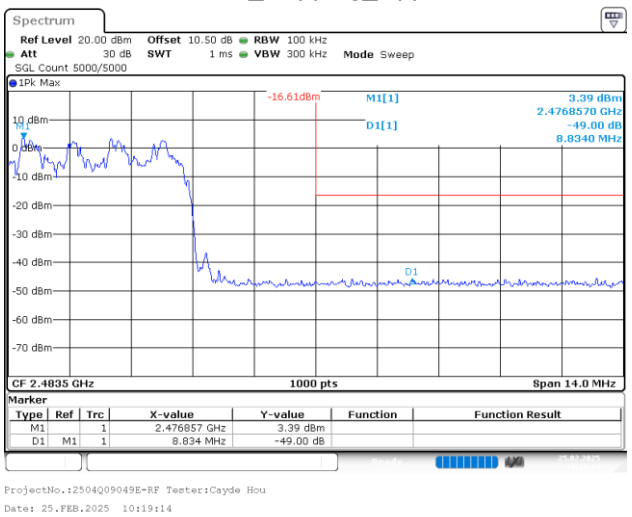
3DH1_High
