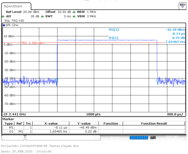
2DH1_Hopping
