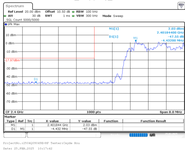
3DH1_Low
