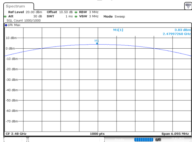
3DH1_High
