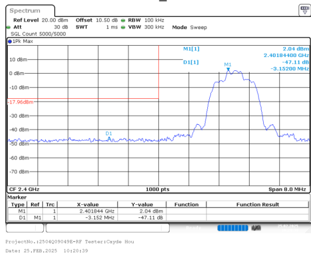
2DH1_Low
