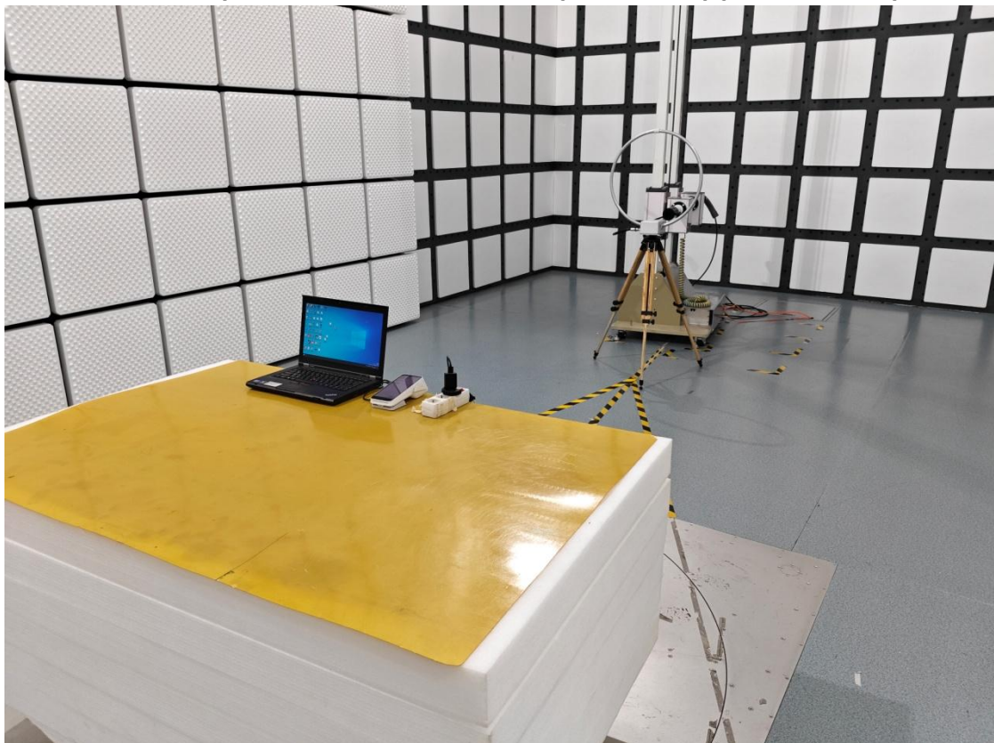
Radiated Spurious Emissions Test View (9kHz-30MHz) (Test Mode 3&4)
