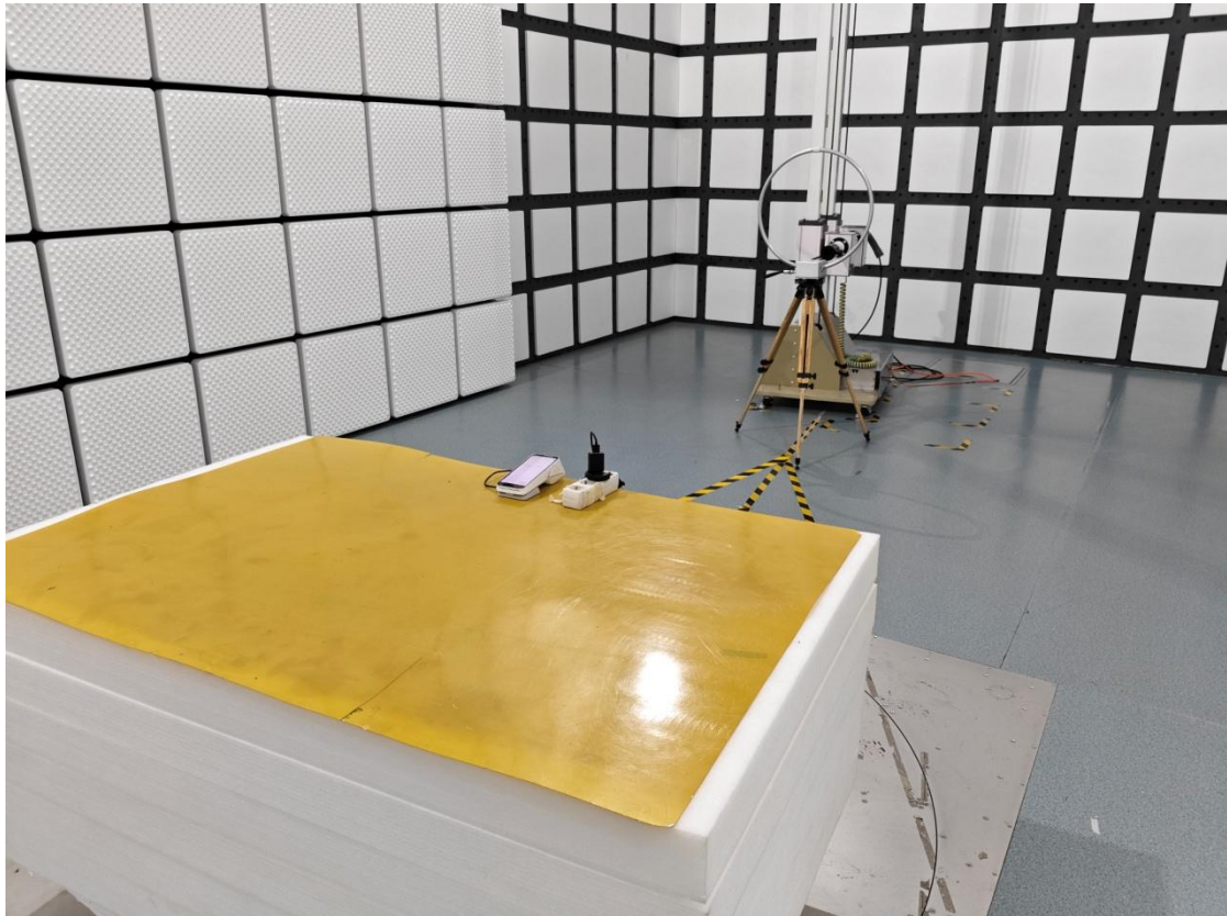
Radiated Spurious Emissions Test View (9kHz-30MHz) (Test Mode 1&2)
