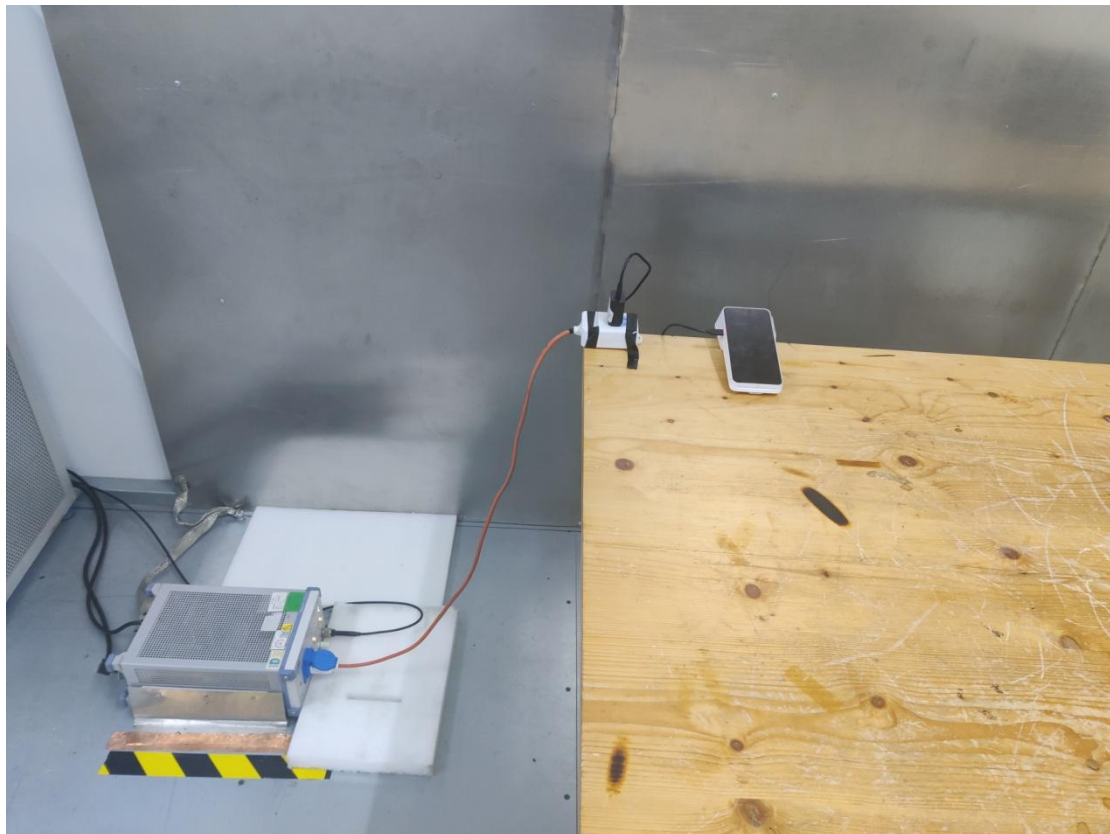
Photo of Power Line Conducted Emission Measurement-Front View(Test Mode 1&2)
