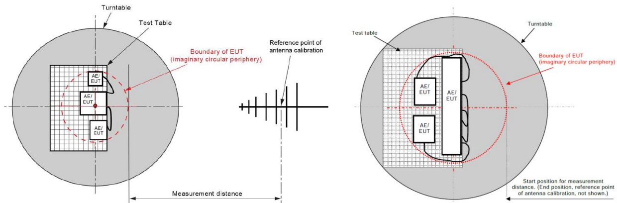
Figure C.1 – Measurement distance
