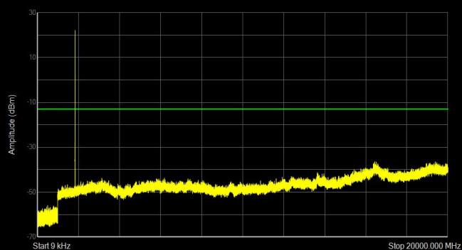
Band25 QPSK BW=1.4MHz Channel=26047 RB Size=6 Position=#0
