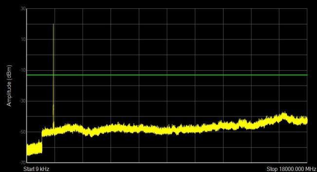
Band4 QPSK BW=3MHz Channel=20175 RB Size=15 Position=#0
