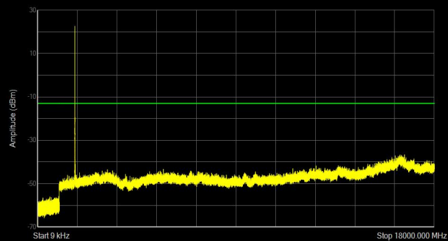
Band4 QPSK BW=3MHz Channel=19965 RB Size=15 Position=#0
