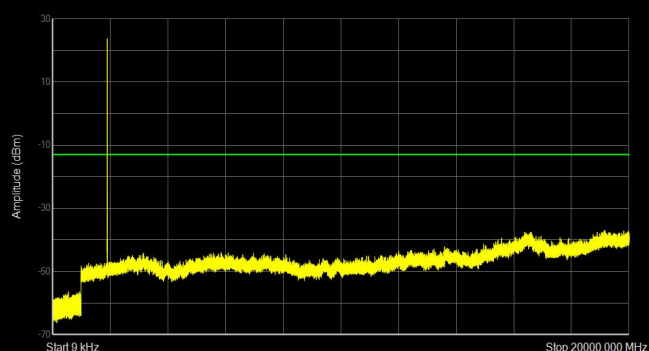
Band25 QPSK BW=1.4MHz Channel=26683 RB Size=6 Position=#0
