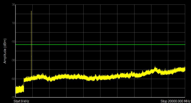
Band25 QPSK BW=1.4MHz Channel=26365 RB Size=6 Position=#0
