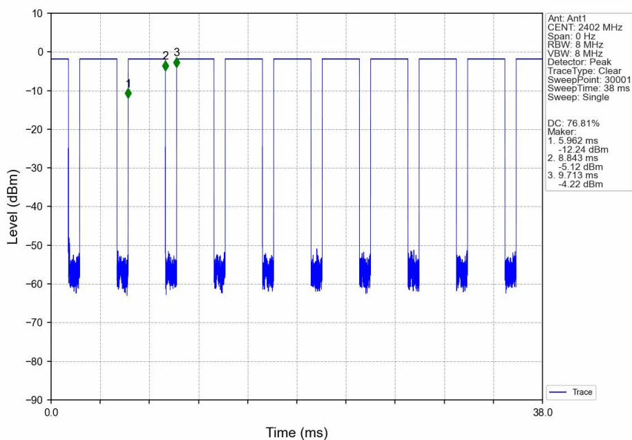
GFSK_DH5_LCH_2402MHz_Ant1_NTNV
