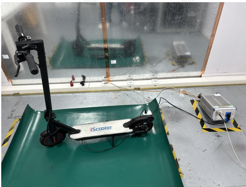
Test Setup Photo of Line Conducted Emissions Measurement
