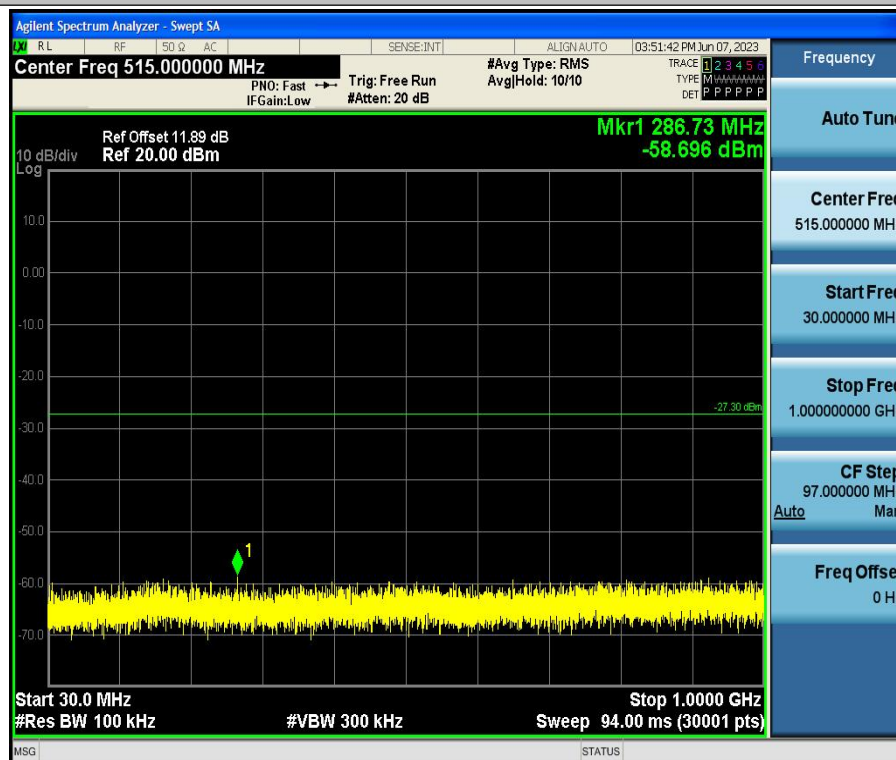
BLE_1M-Ant1-2402-0~Reference
