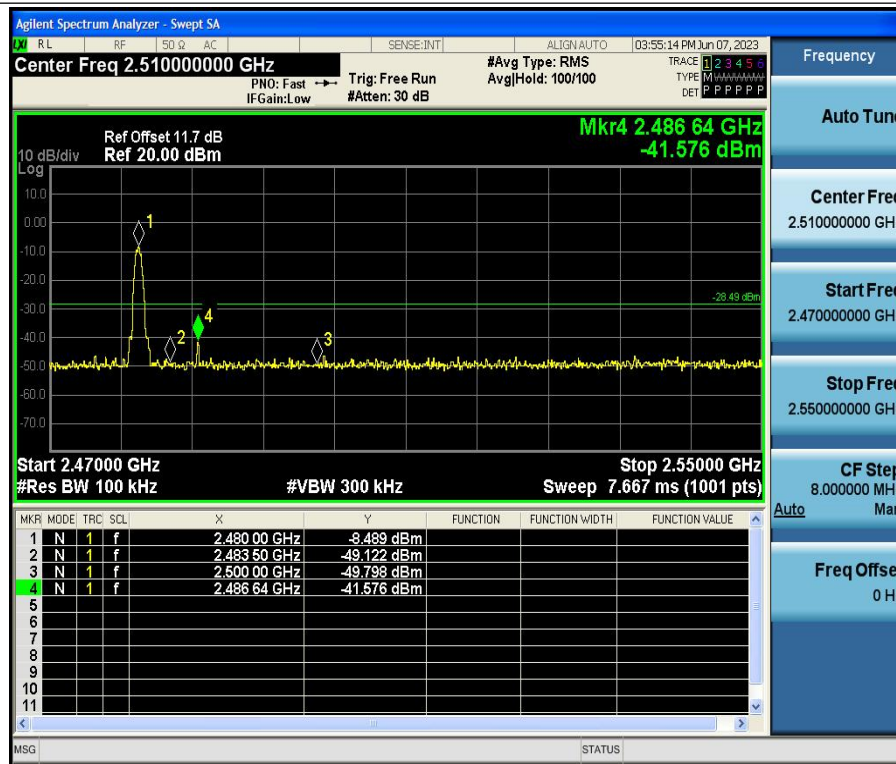
BLE_1M-Ant1-2480
