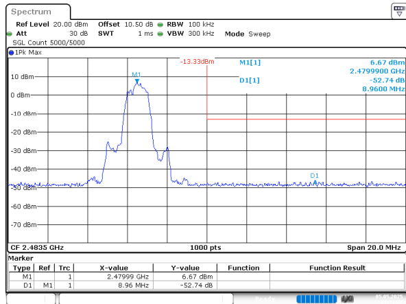
2EDR_DH1_High
