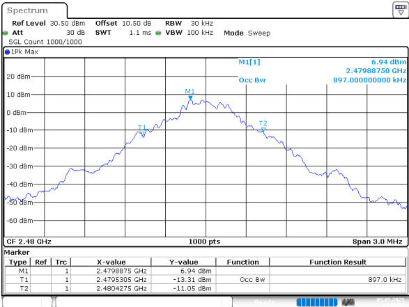
BDR_DH1_High
