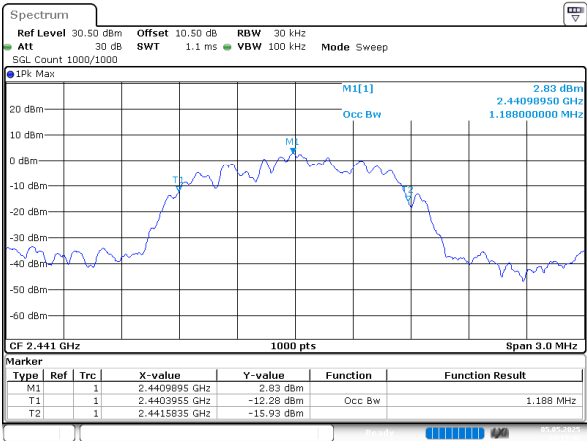
2EDR_DH1_Middle
