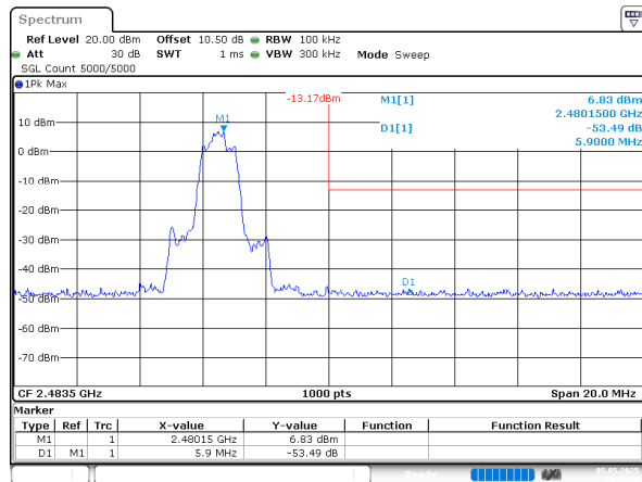
3EDR_DH1_High
