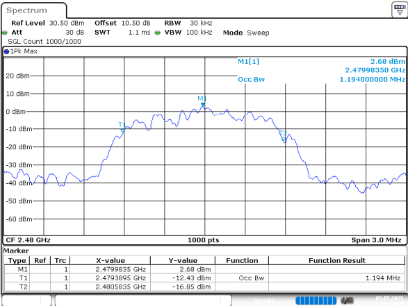
2EDR_DH1_High
