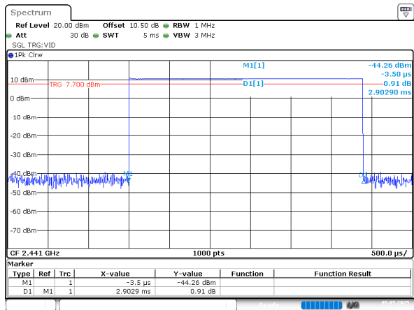
BDR_DH5_Hopping
