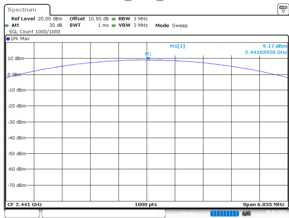
3EDR_DH1_Middle
