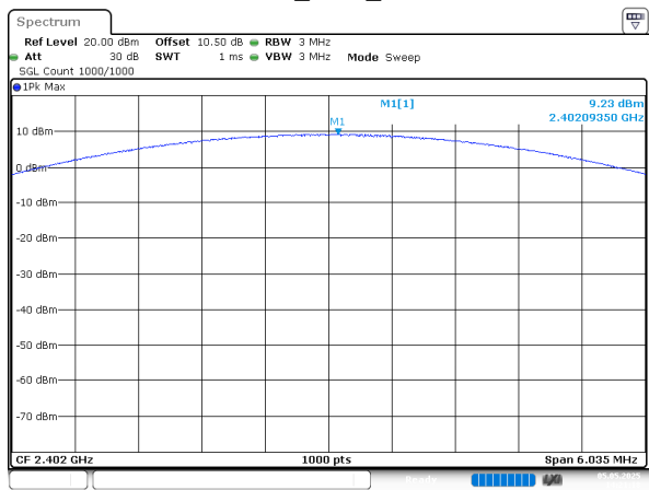
3EDR_DH1_Low
