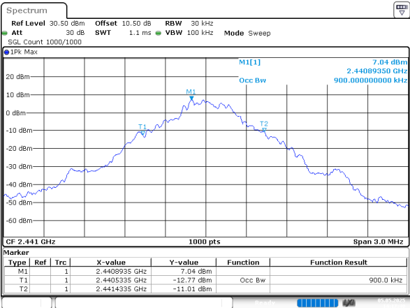
BDR_DH1_Middle
