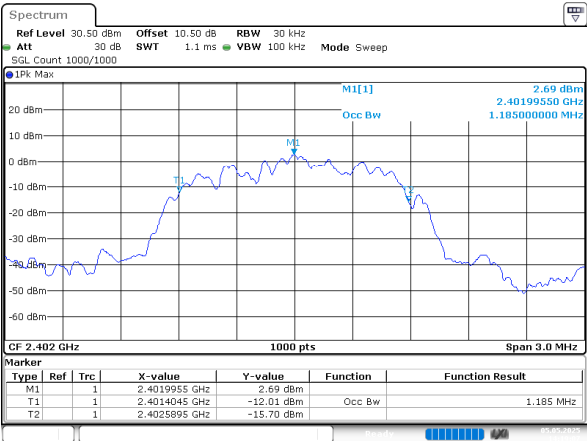
2EDR_DH1_Low
