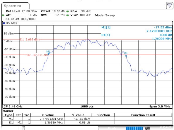
2EDR_DH1_High
