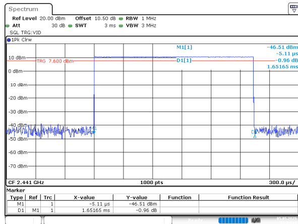
BDR_DH3_Hopping
