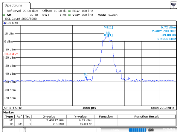
3EDR_DH1_Low
