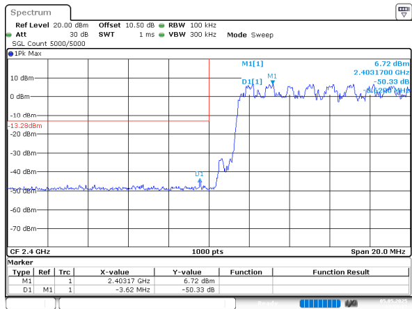
3EDR_DH1_Hopping_Lower
