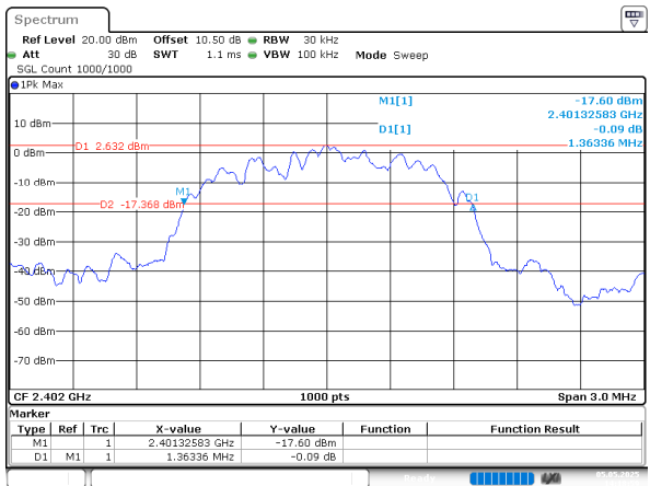
2EDR_DH1_Low
