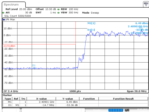
2EDR_DH1_Hopping_Lower
