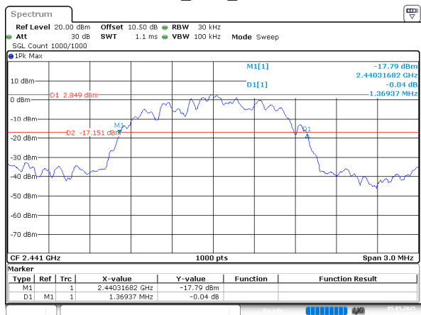
2EDR_DH1_Middle
