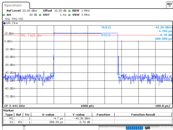
BDR_DH1_Hopping
