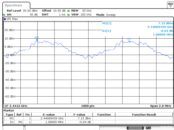
BDR_DH1_Middle
