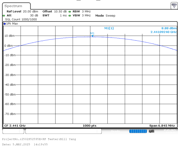
2EDR_DH1_Middle
