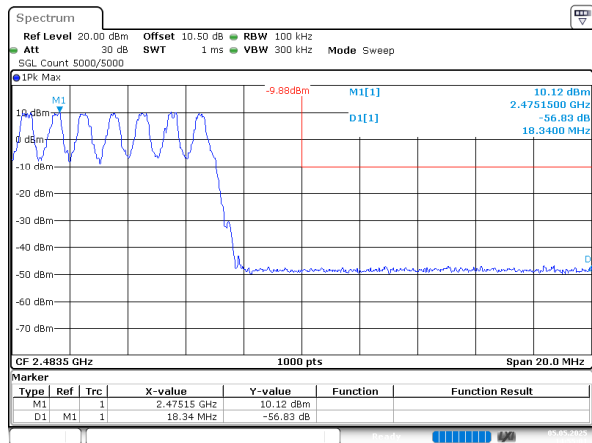
BDR_DH1_Hopping_Upper
