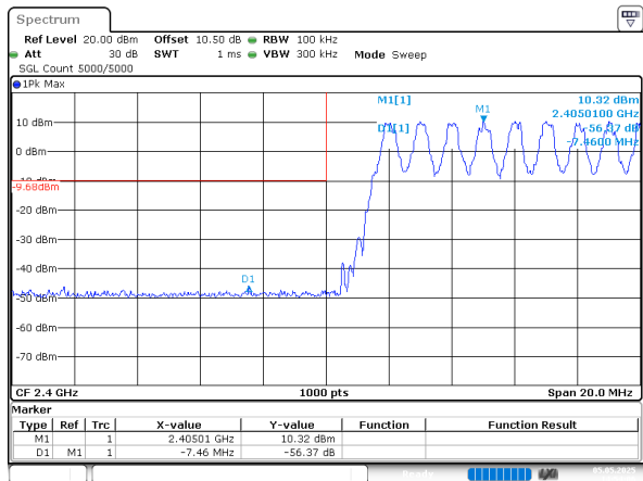
BDR_DH1_Hopping_Lower
