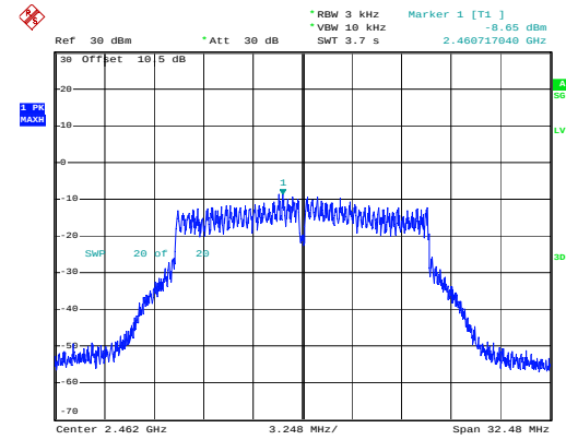
802.11g_2462MHz
