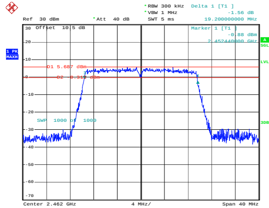
802.11ax20_2462MHz
