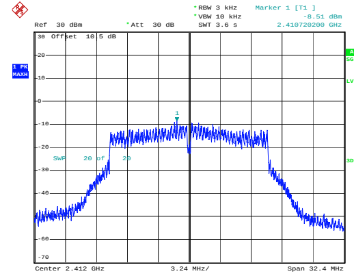
802.11g_2412MHz
