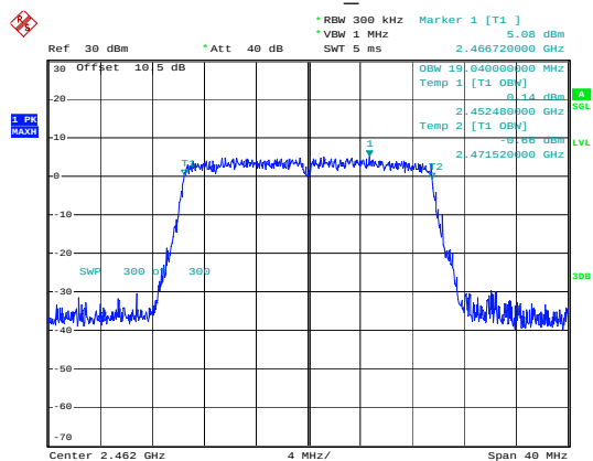
802.11ax20_2462MHz
