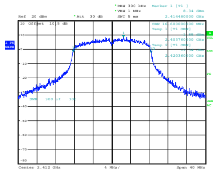
g_2412MHz_Chain 0
