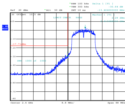
n20_2412MHz_Chain 0
