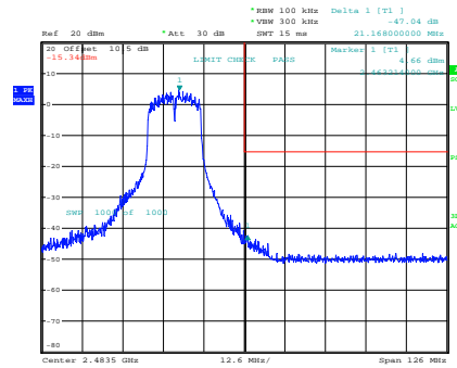
g_2462MHz_Chain 0
