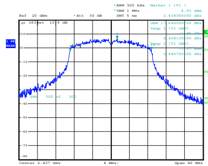
n20_2437MHz_Chain 0
