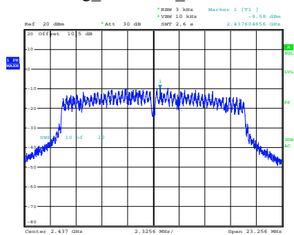
g_2437MHz_Chain 0
