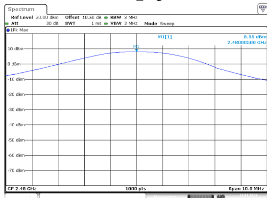
GFSK_High
