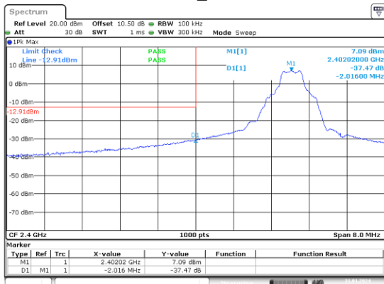
GFSK_Low
