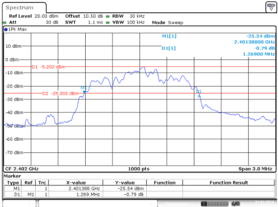
8DPSK_Low
