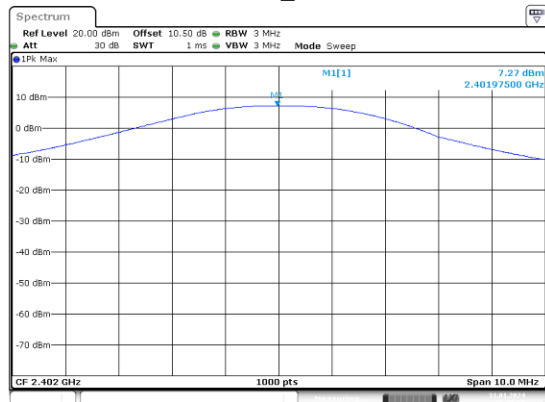
GFSK_Low
