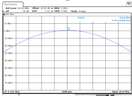
8DPSK_Middle
