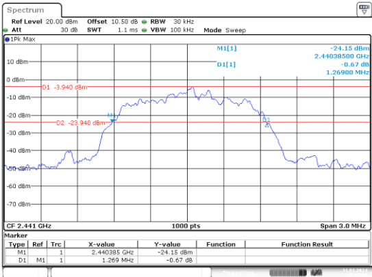
8DPSK_Middle
