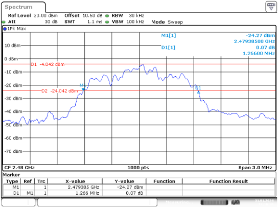
8DPSK_High
