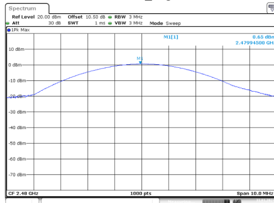
8DPSK_High
