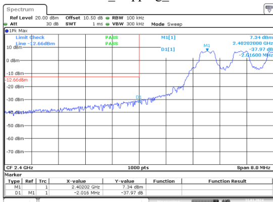
GFSK_Hopping_Lower
