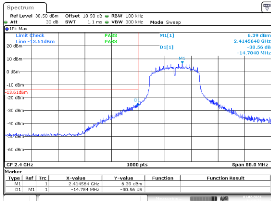
g_2412MHz
