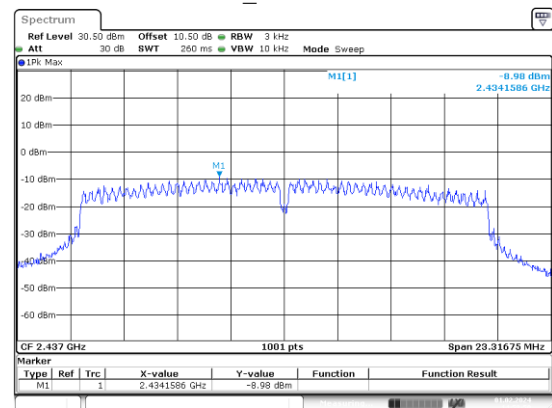
n20_2437MHz
