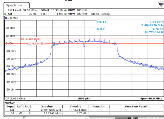
g_2412MHz
