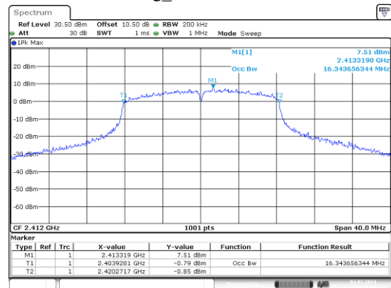
g_2412MHz
