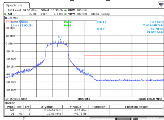
n20_2462MHz_
