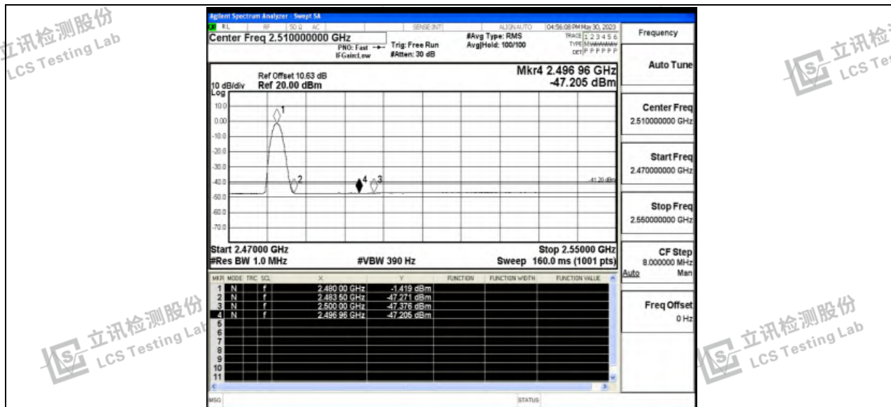
3DH5_Ant1_High_2480_Peak
