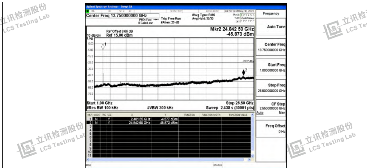
3DH5_Ant1_2441_0~Reference
