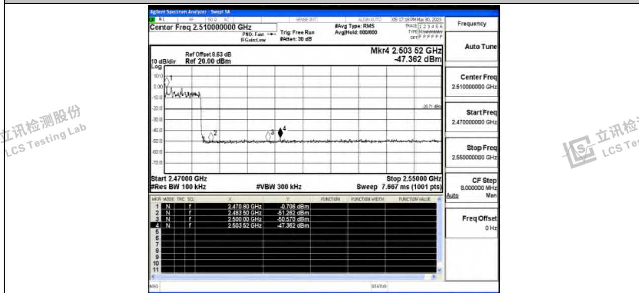
3DH5_Ant1_High_Hop_2480
