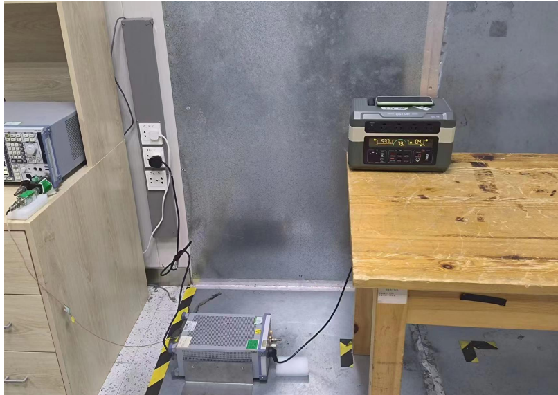
Conducted Emissions
