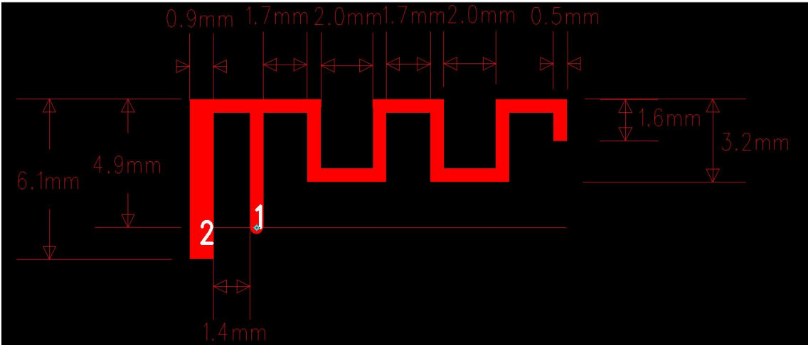
Model: Plannar Inverted F Antenna on board
