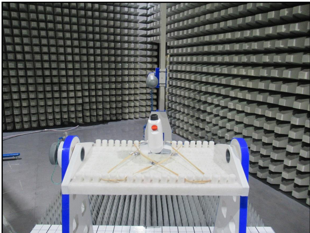
Photo 6: Radiated Test Setup from 30 MHz to 1 GHz
