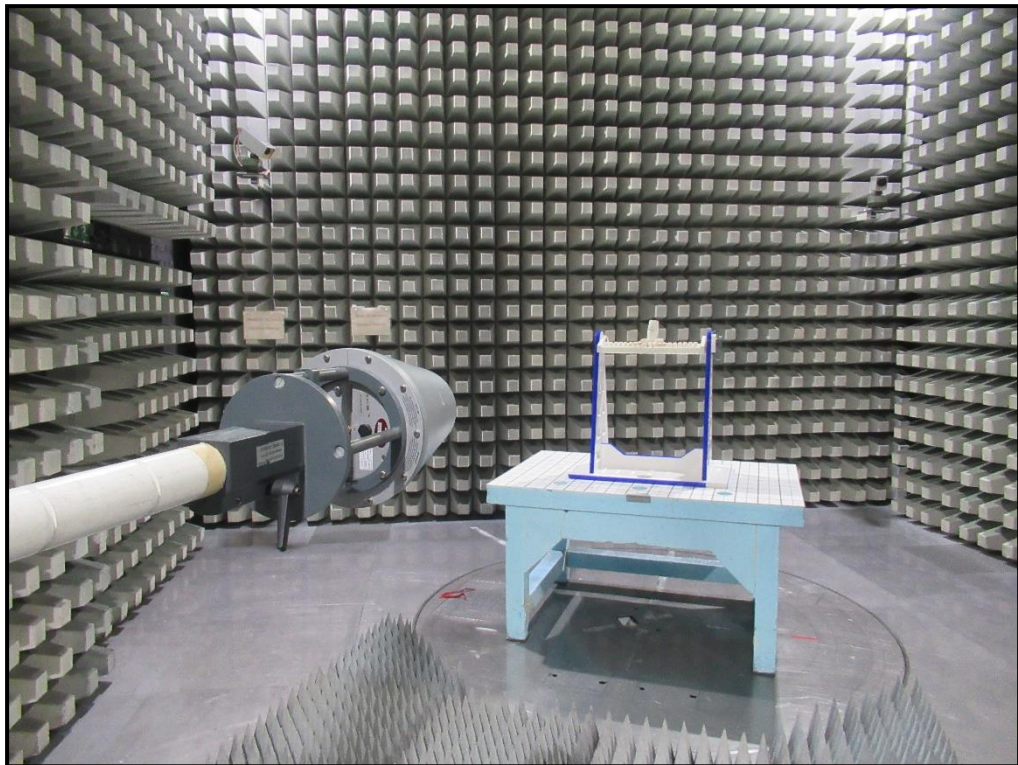
Photo 5: Radiated Test Setup from 30 MHz to 1 GHz
