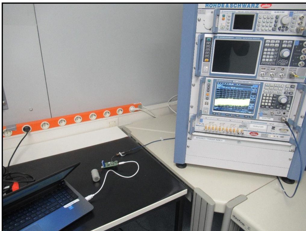
Photo 8: Conducted Test Setup
