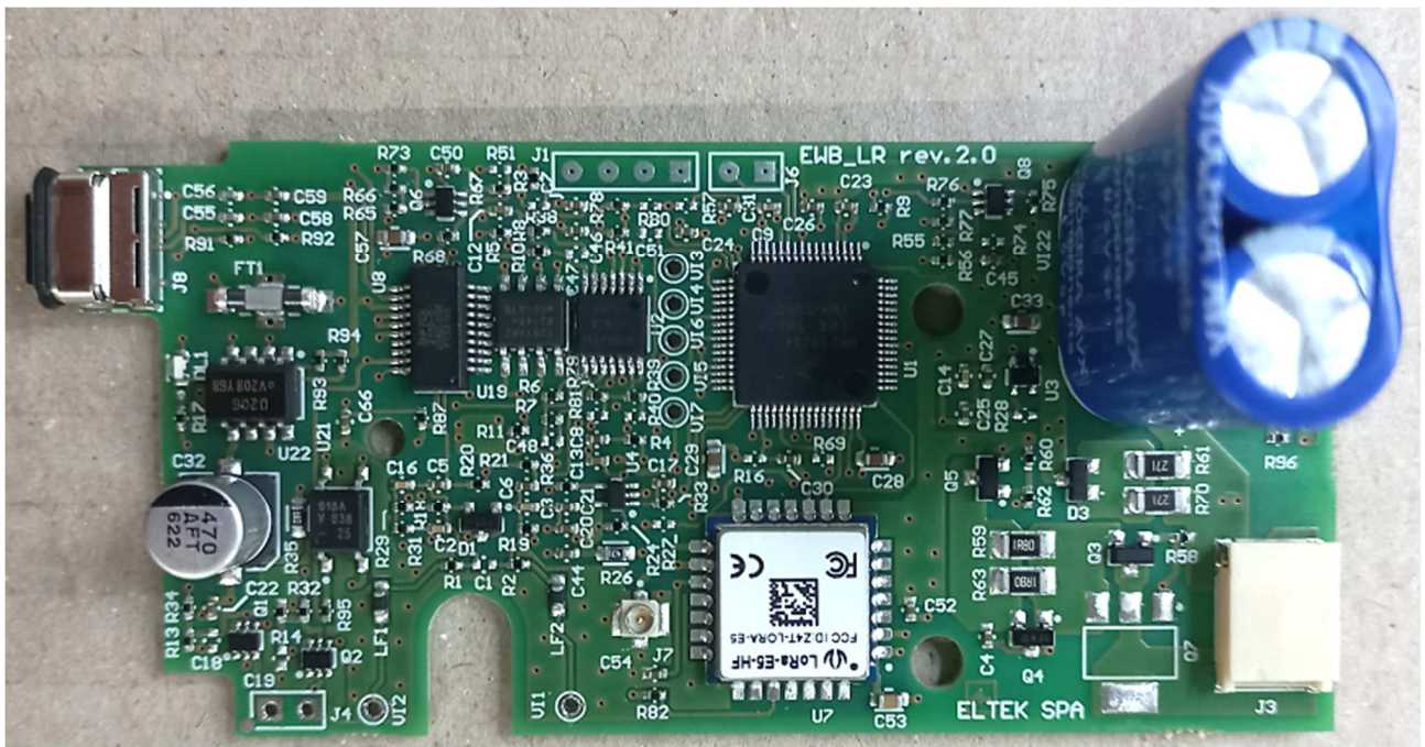
LoRa pcb - Top (component) view
