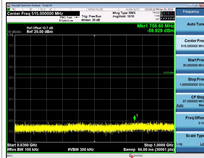
30MHz-1G
