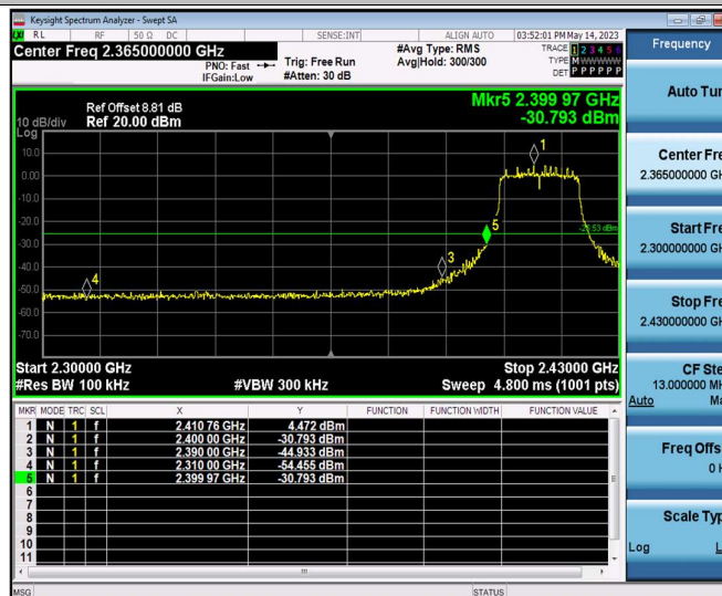
11N20SISO_Ant1_Low_2412
