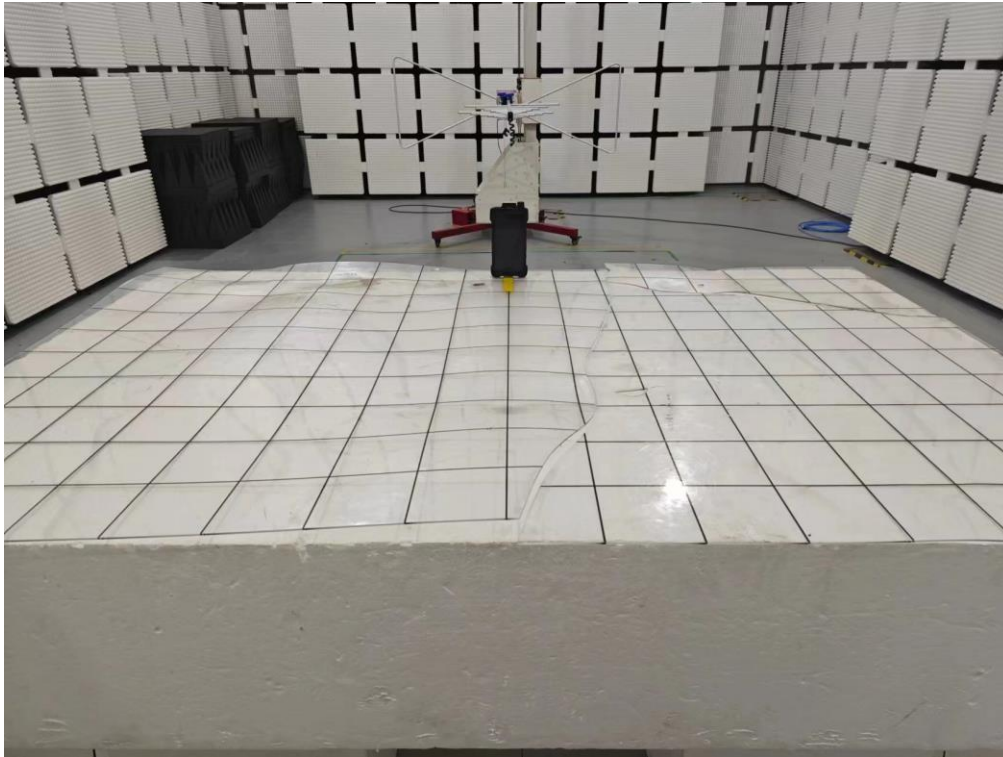
Radiated Spurious Emission Test Setup Photo – 30-1000MHz
