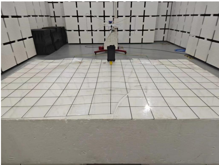
Radiated Spurious Emission Test Setup Photo – 30-1000MHz
