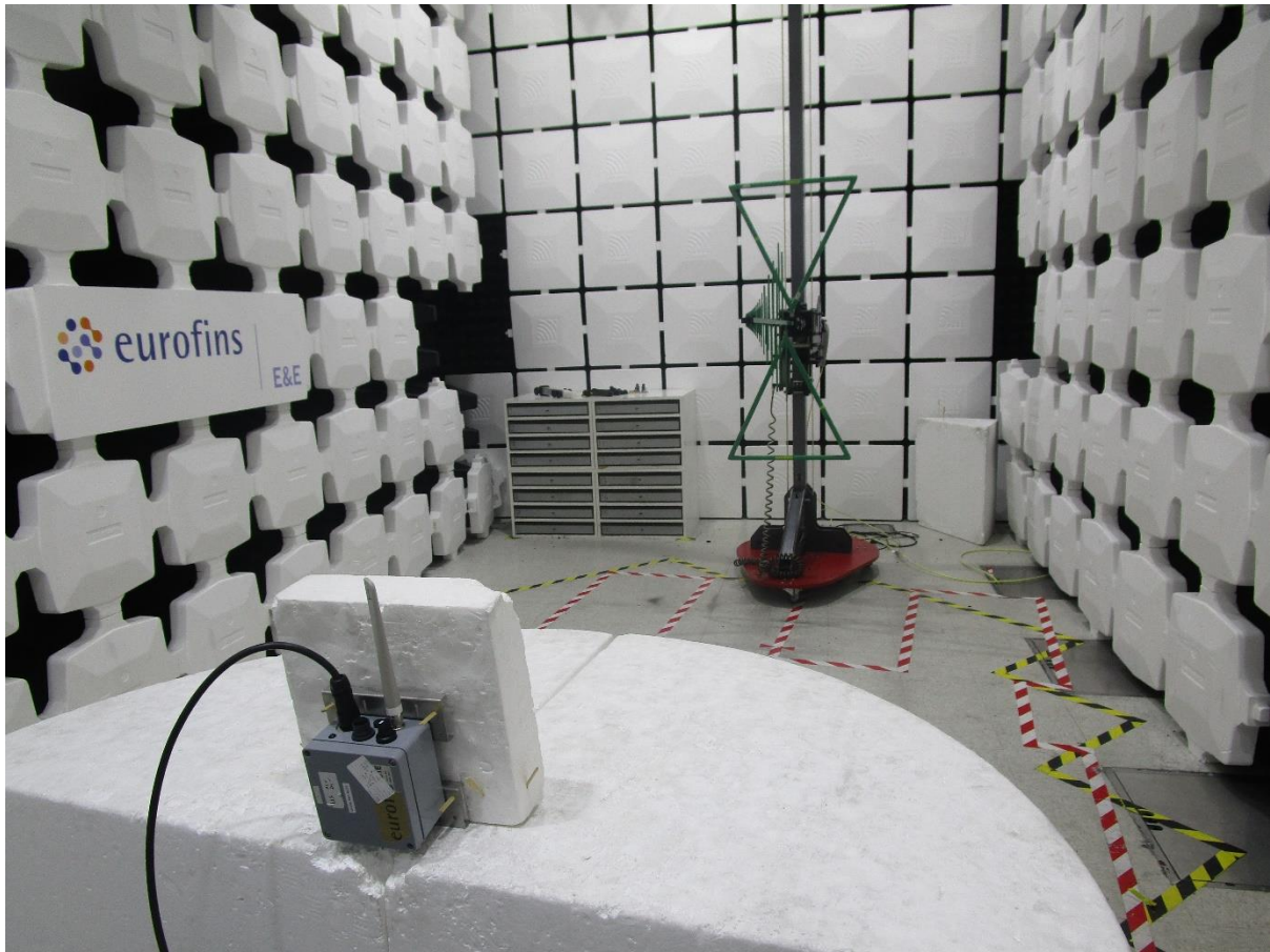
Radiated tests 30MHz to 1GHz
