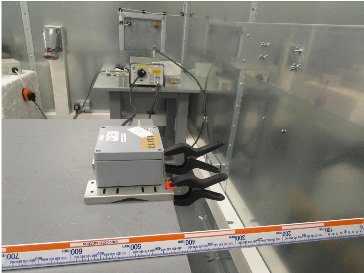
Mains conducted emissions test set up end view
