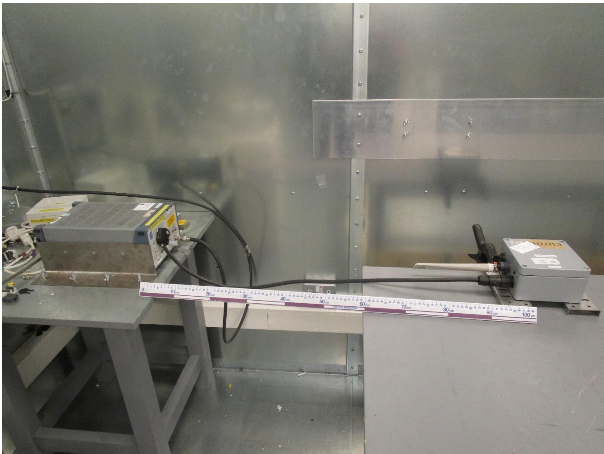
Mains conducted emissions test set up side view
