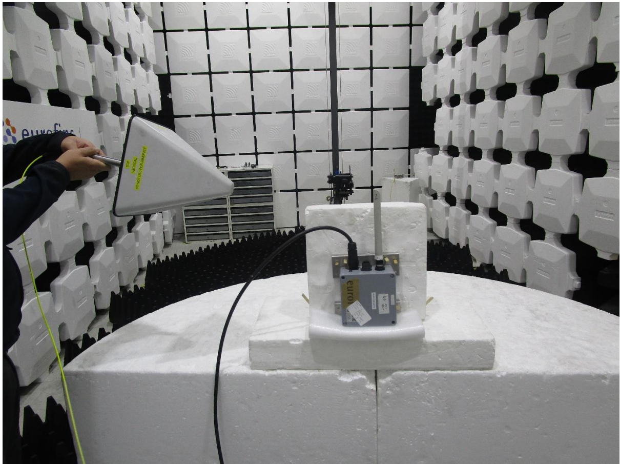
Investigative measurements 1-18GHz
