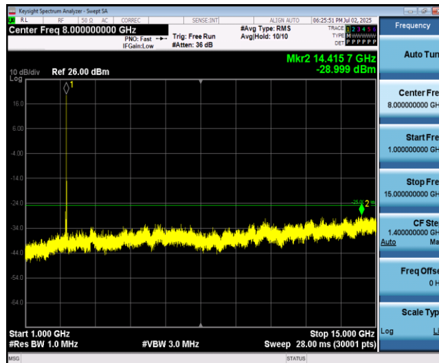
Band41-20MHz-16QAM-41140-1RB#0-Range2:1000~15000MHz
