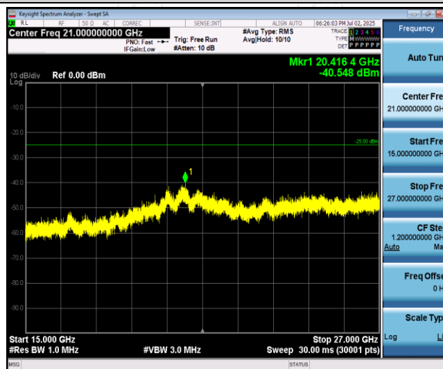
Band41-20MHz-16QAM-41140-1RB#0-Range3:15000~27000MHz
