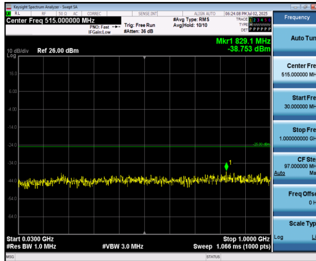
Band41-20MHz-16QAM-40690-1RB#0-Range1:30~1000MHz
