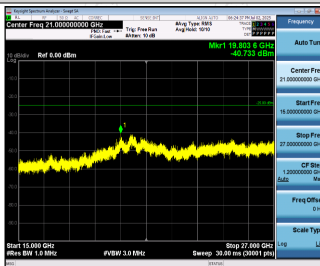
Band41-20MHz-16QAM-40690-1RB#0-Range3:15000~27000MHz
