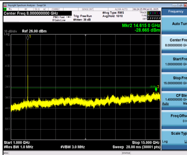
Band41-20MHz-16QAM-40690-1RB#0-Range2:1000~15000MHz
