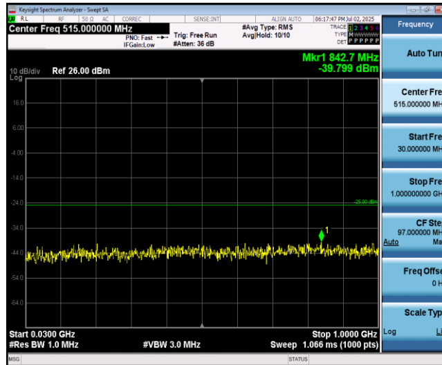
Band41-15MHz-QPSK-40690-1RB#0-Range1:30~1000MHz
