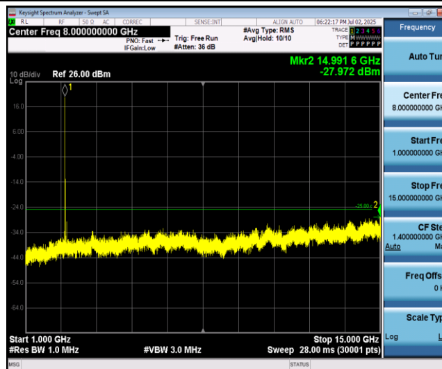
Band41-20MHz-QPSK-40340-1RB#0-Range2:1000~15000MHz
