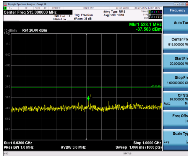
Band41-20MHz-16QAM-40340-1RB#0-Range1:30~1000MHz
