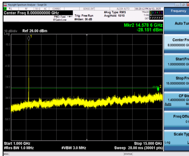
Band41-15MHz-16QAM-41165-1RB#0-Range2:1000~15000MHz
