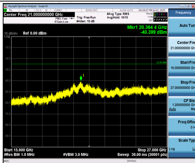
Band41-5MHz-16QAM-41215-1RB#0-Range3:15000~27000MHz
