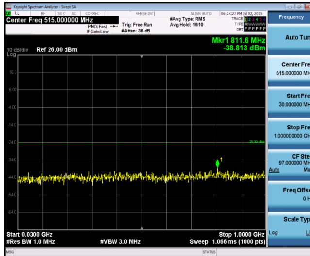
Band41-20MHz-QPSK-40690-1RB#0-Range1:30~1000MHz
