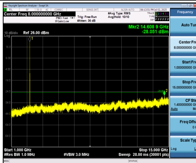
Band41-10MHz-QPSK-41190-1RB#0-Range2:1000~15000MHz
