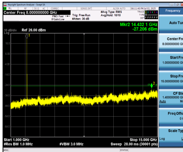
Band41-10MHz-16QAM-40290-1RB#0-Range2:1000~15000MHz
