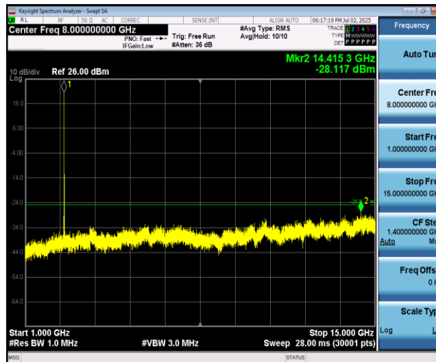
Band41-15MHz-16QAM-40315-1RB#0-Range2:1000~15000MHz
