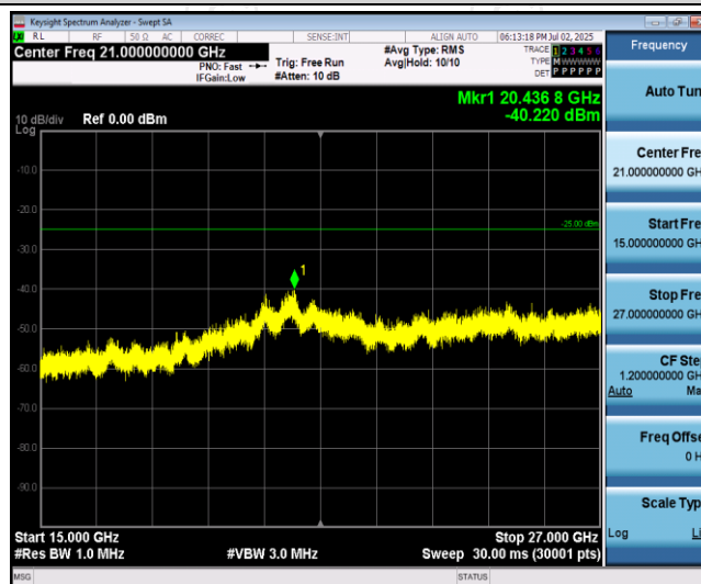
Band41-10MHz-16QAM-40690-1RB#0-Range3:15000~27000MHz
