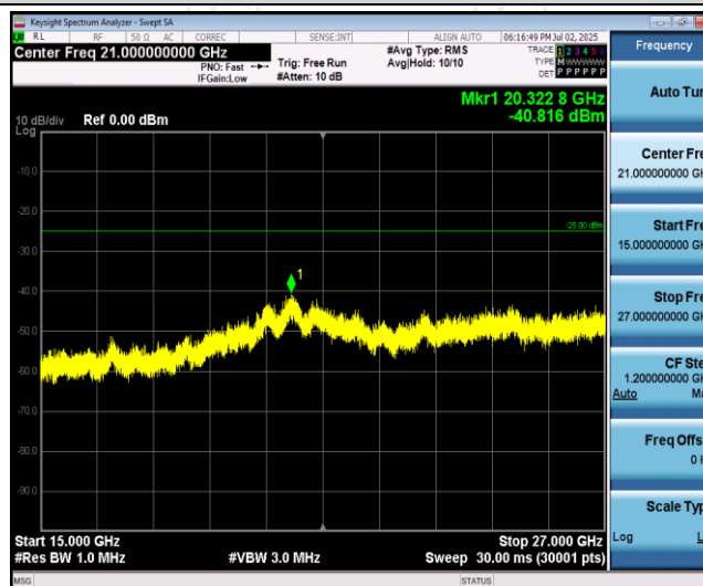
Band41-15MHz-QPSK-40315-1RB#0-Range3:15000~27000MHz
