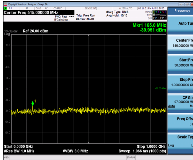
Band41-15MHz-QPSK-40315-1RB#0-Range1:30~1000MHz
