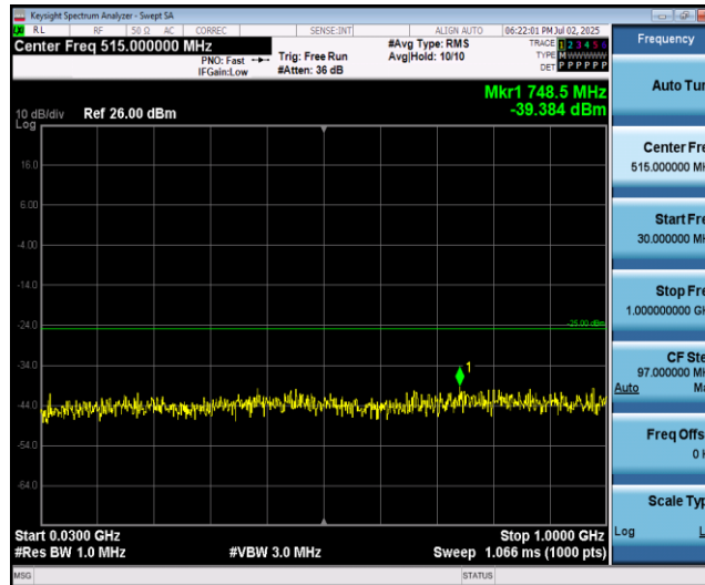
Band41-20MHz-QPSK-40340-1RB#0-Range1:30~1000MHz
