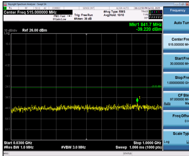
Band41-10MHz-16QAM-40690-1RB#0-Range1:30~1000MHz
