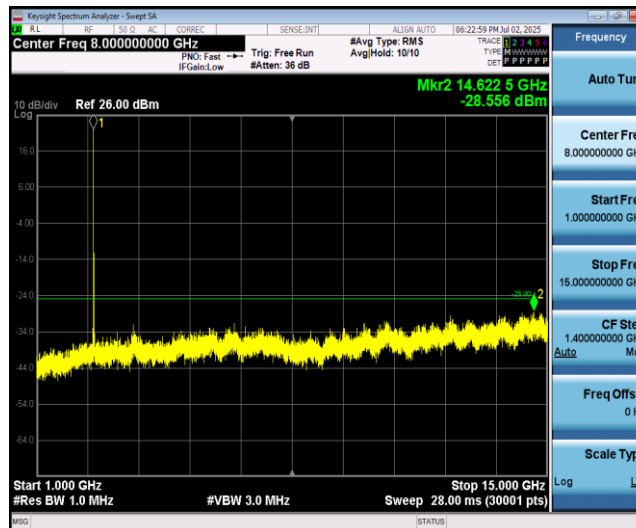
Band41-20MHz-16QAM-40340-1RB#0-Range2:1000~15000MHz
