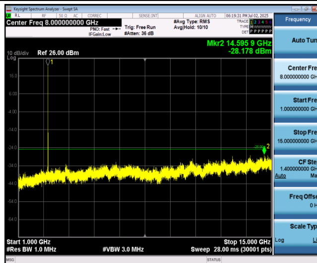
Band41-15MHz-QPSK-41165-1RB#0-Range2:1000~15000MHz
