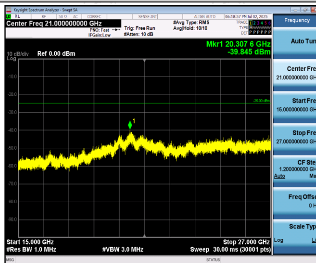
Band41-15MHz-16QAM-40690-1RB#0-Range3:15000~27000MHz
