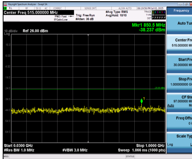
Band41-15MHz-16QAM-41165-1RB#0-Range1:30~1000MHz
