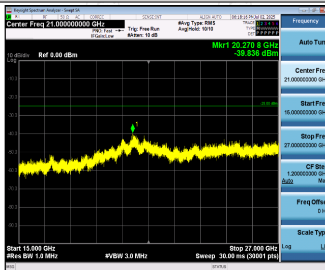
Band41-15MHz-QPSK-40690-1RB#0-Range3:15000~27000MHz
