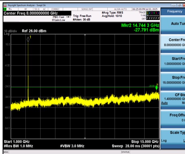
Band41-20MHz-QPSK-41140-1RB#0-Range2:1000~15000MHz
