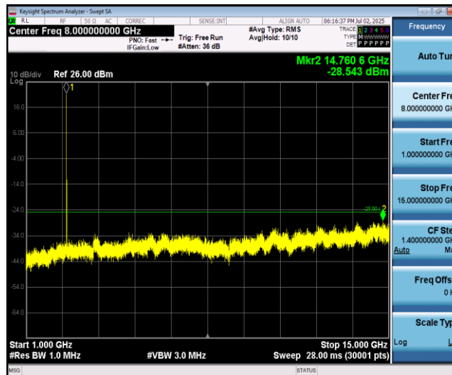
Band41-15MHz-QPSK-40315-1RB#0-Range2:1000~15000MHz
