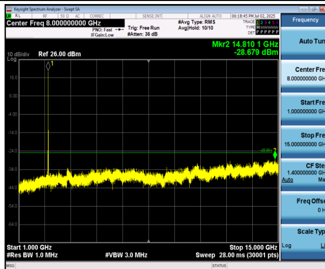
Band41-15MHz-16QAM-40690-1RB#0-Range2:1000~15000MHz
