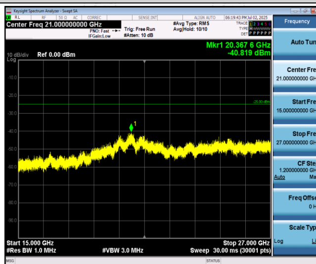
Band41-15MHz-QPSK-41165-1RB#0-Range3:15000~27000MHz
