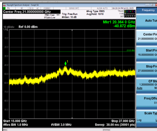
Band41-15MHz-16QAM-41165-1RB#0-Range3:15000~27000MHz
