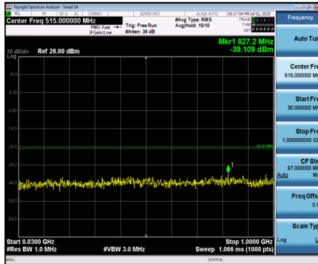
Band41-15MHz-16QAM-40315-1RB#0-Range1:30~1000MHz
