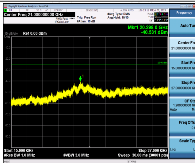
Band41-20MHz-16QAM-40340-1RB#0-Range3:15000~27000MHz
