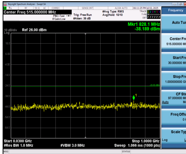
Band41-10MHz-16QAM-40290-1RB#0-Range1:30~1000MHz
