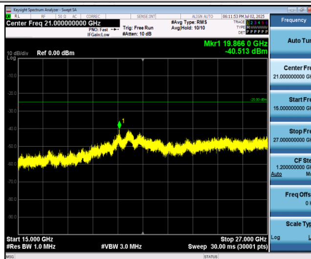
Band41-10MHz-16QAM-40290-1RB#0-Range3:15000~27000MHz
