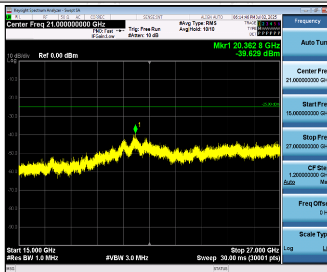
Band41-10MHz-16QAM-41190-1RB#0-Range3:15000~27000MHz
