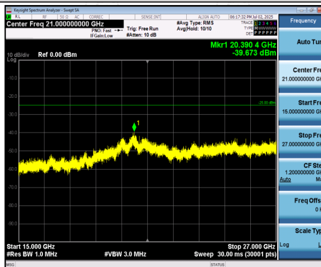
Band41-15MHz-16QAM-40315-1RB#0-Range3:15000~27000MHz
