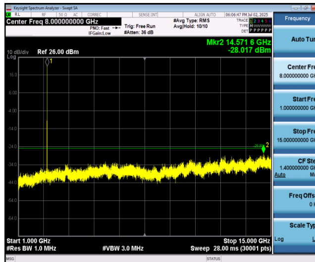
Band41-5MHz-QPSK-40690-1RB#0-Range2:1000~15000MHz
