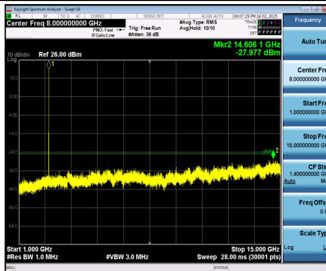
Band41-5MHz-16QAM-40690-1RB#0-Range2:1000~15000MHz
