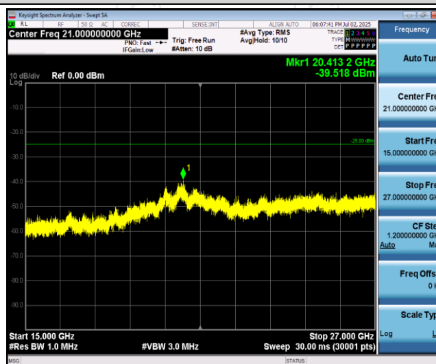
Band41-5MHz-16QAM-40690-1RB#0-Range3:15000~27000MHz
