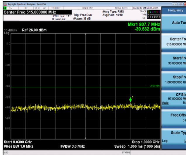
Band41-5MHz-16QAM-40690-1RB#0-Range1:30~1000MHz
