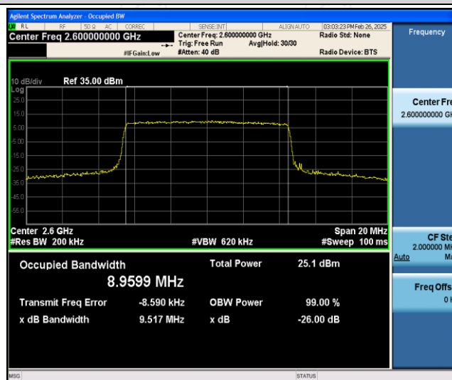
Band41-10MHz-QPSK-40690-50RB#0
