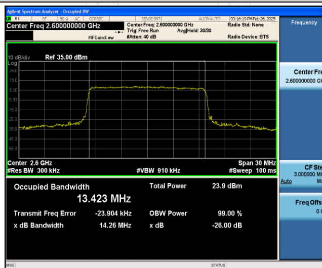
Band41-15MHz-16QAM-40690-75RB#0
