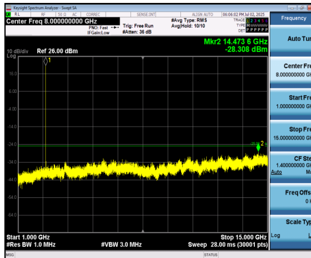
Band41-5MHz-16QAM-40265-1RB#0-Range2:1000~15000MHz
