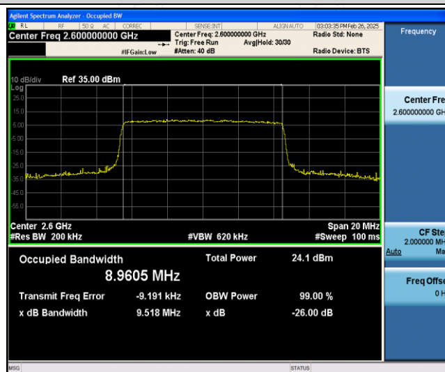
Band41-10MHz-16QAM-40690-50RB#0
