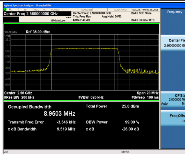
Band41-10MHz-QPSK-40290-50RB#0
