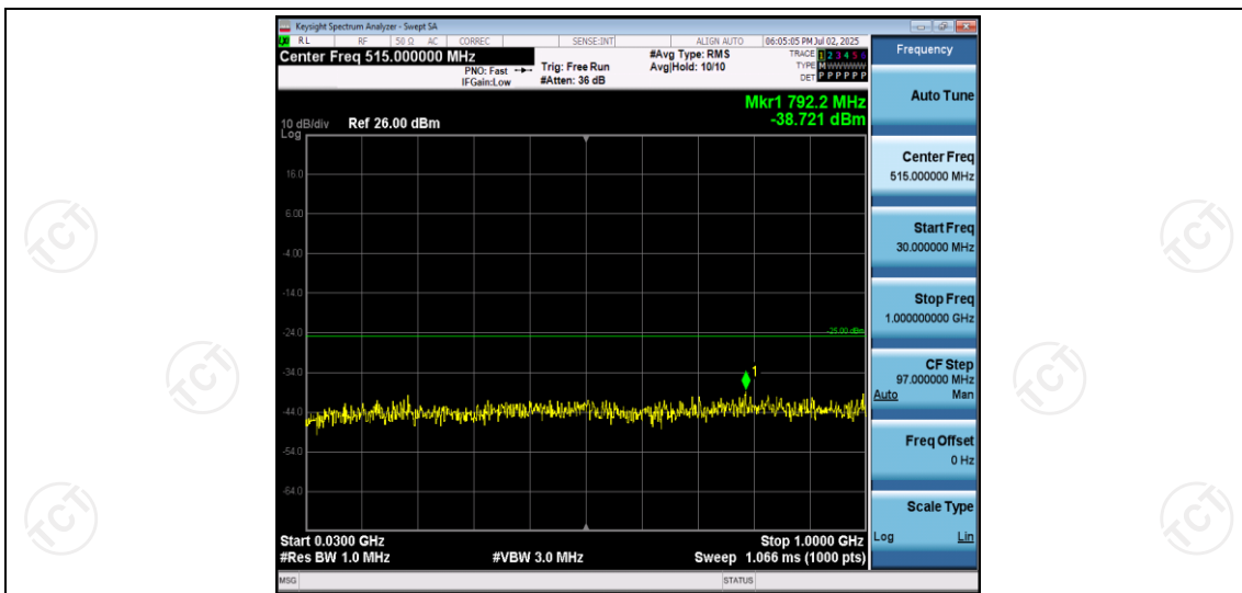
Band41-5MHz-QPSK-40265-1RB#0-Range1:30~1000MHz
