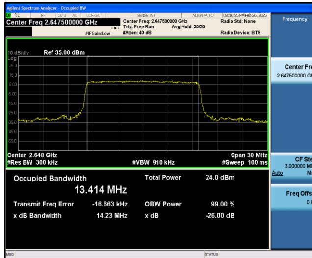
Band41-15MHz-QPSK-41165-75RB#0
