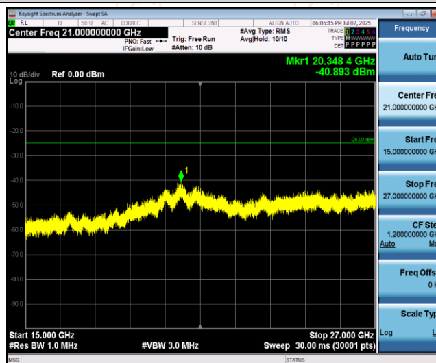
Band41-5MHz-16QAM-40265-1RB#0-Range3:15000~27000MHz
