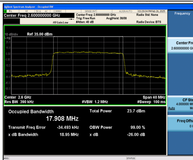
Band41-20MHz-16QAM-40690-100RB#0
