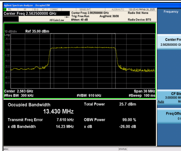
Band41-15MHz-QPSK-40315-75RB#0
