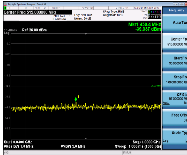
Band41-5MHz-16QAM-40265-1RB#0-Range1:30~1000MHz
