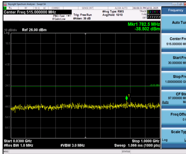
Band41-5MHz-QPSK-40690-1RB#0-Range1:30~1000MHz
