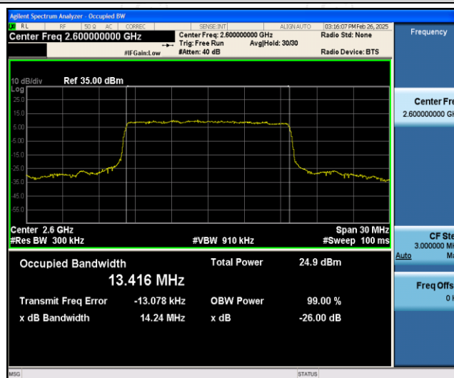
Band41-15MHz-QPSK-40690-75RB#0
