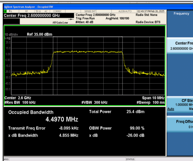
Band41-5MHz-16QAM-40690-25RB#0
