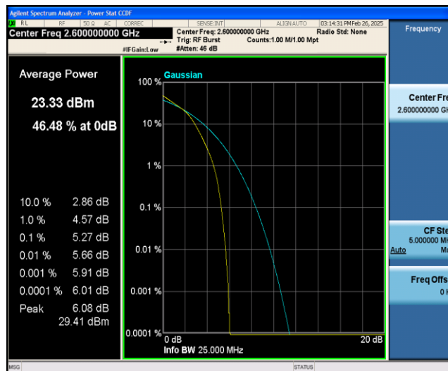
Band41-10MHz-16QAM-40690-50RB#0
