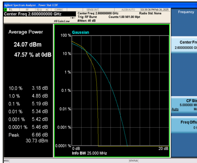
Band41-20MHz-16QAM-40690-1RB#0
