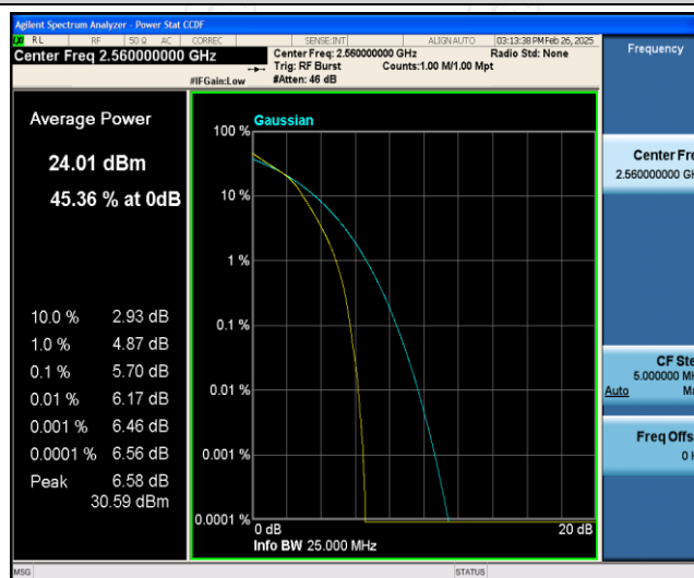
Band41-10MHz-16QAM-40290-50RB#0
