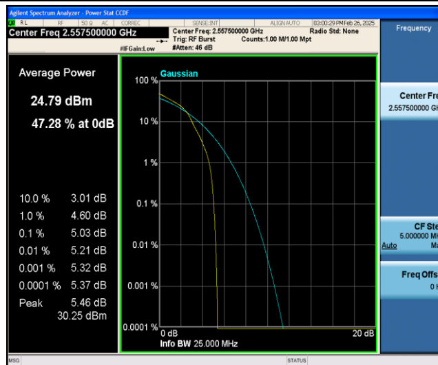
Band41-5MHz-16QAM-40265-1RB#0
