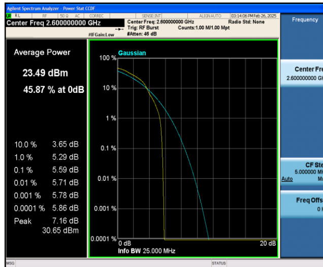
Band41-10MHz-16QAM-40690-1RB#0
