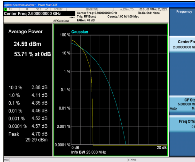
Band41-5MHz-QPSK-40690-1RB#0
