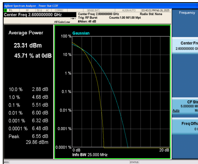
Band41-20MHz-16QAM-40690-100RB#0
