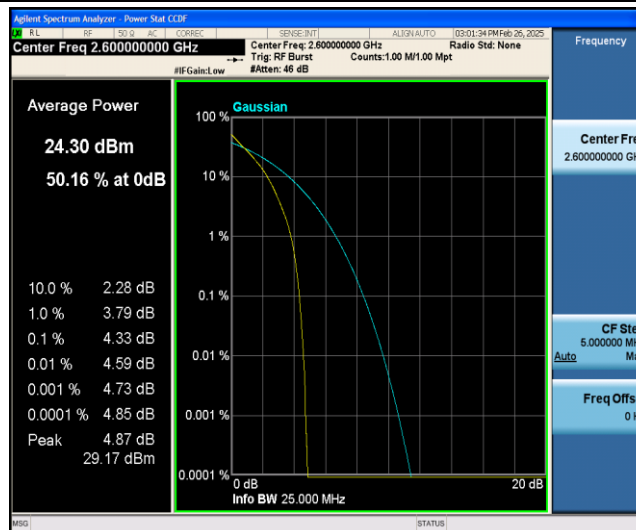
Band41-5MHz-QPSK-40690-25RB#0
