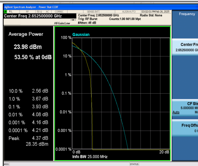
Band41-5MHz-QPSK-41215-1RB#0
