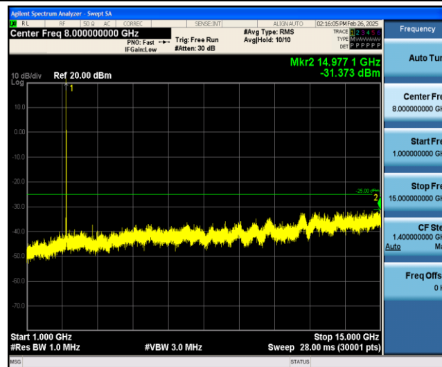
Band7-10MHz-16QAM-21400-1RB#0-Range2:1000~15000MHz
