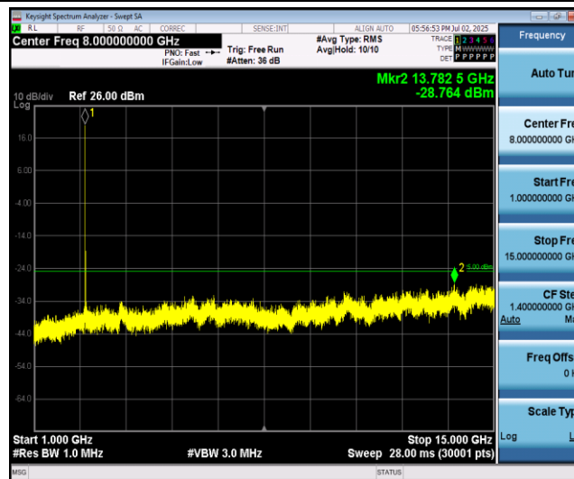
Band7-15MHz-16QAM-21375-1RB#0-Range2:1000~15000MHz
