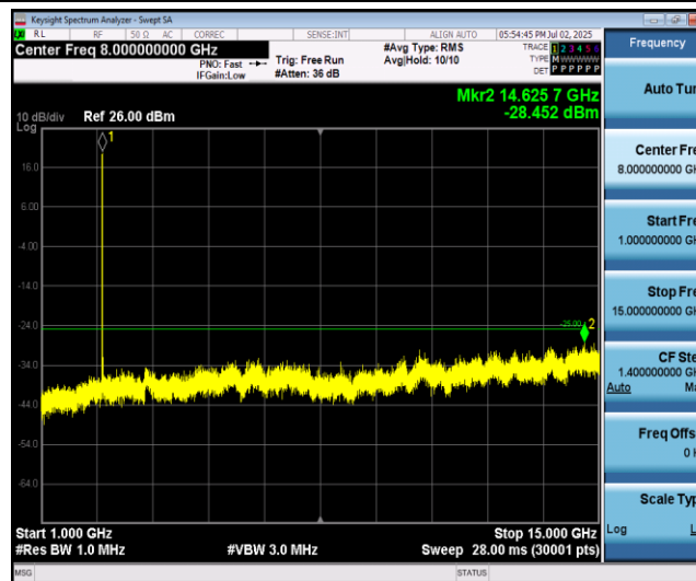
Band7-15MHz-QPSK-21100-1RB#0-Range2:1000~15000MHz
