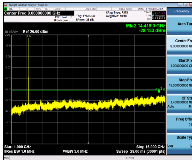
Band7-15MHz-QPSK-21375-1RB#0-Range2:1000~15000MHz
