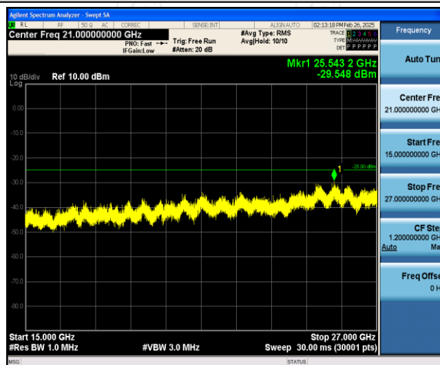
Band7-10MHz-16QAM-20800-1RB#0-Range3:15000~27000MHz
