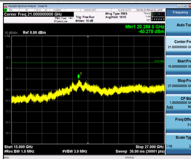
Band7-15MHz-QPSK-21375-1RB#0-Range3:15000~27000MHz
