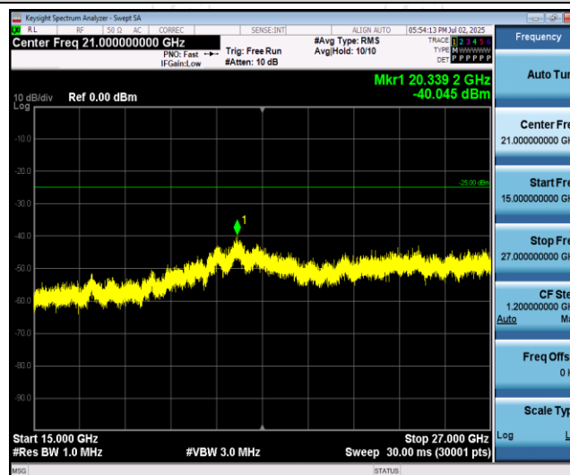
Band7-15MHz-16QAM-20825-1RB#0-Range3:15000~27000MHz
