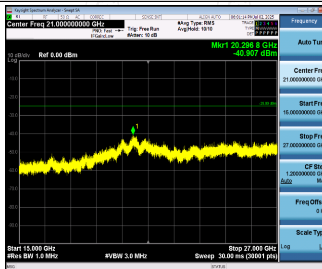
Band7-20MHz-16QAM-21100-1RB#0-Range3:15000~27000MHz
