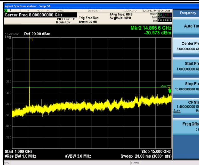
Band7-10MHz-QPSK-21100-1RB#0-Range2:1000~15000MHz
