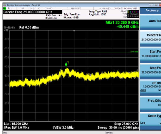
Band7-15MHz-QPSK-21100-1RB#0-Range3:15000~27000MHz
