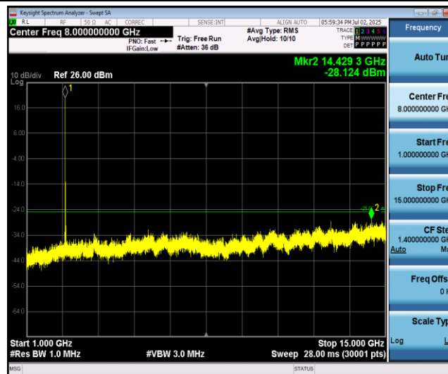
Band7-20MHz-16QAM-20850-1RB#0-Range2:1000~15000MHz
