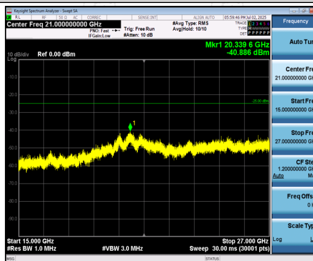
Band7-20MHz-16QAM-20850-1RB#0-Range3:15000~27000MHz
