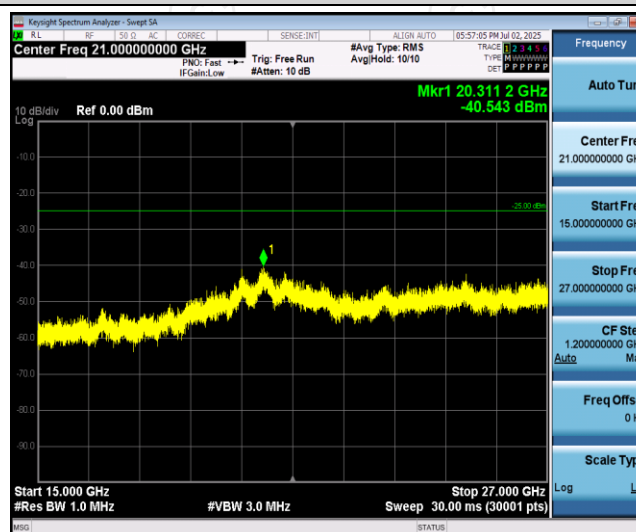
Band7-15MHz-16QAM-21375-1RB#0-Range3:15000~27000MHz
