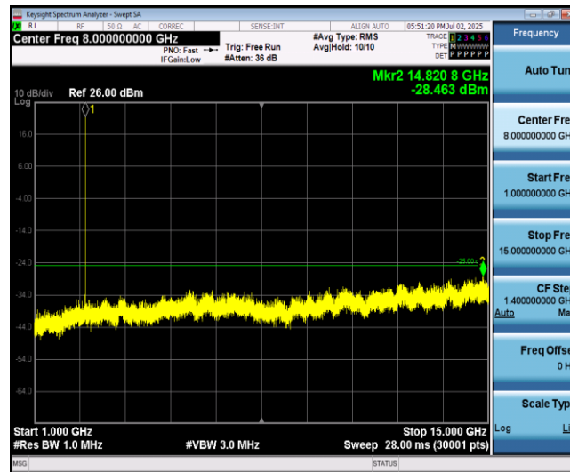
Band7-5MHz-16QAM-21425-1RB#0-Range2:1000~15000MHz
