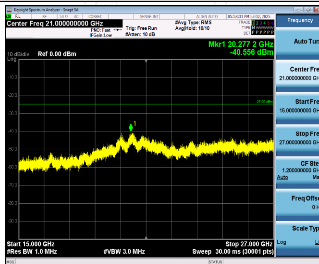
Band7-15MHz-QPSK-20825-1RB#0-Range3:15000~27000MHz
