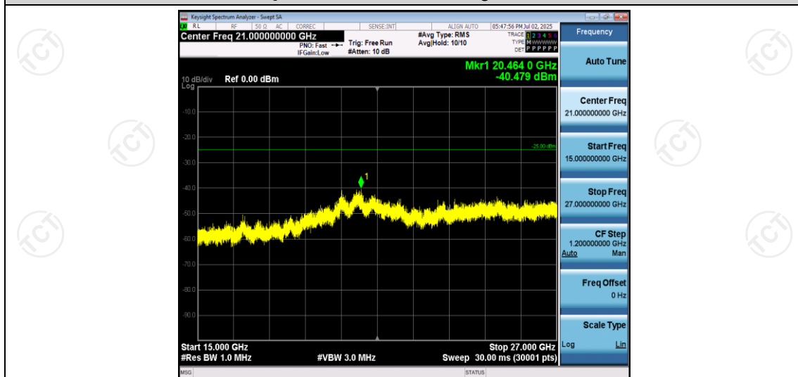
Band7-5MHz-QPSK-20775-1RB#0-Range3:15000~27000MHz
