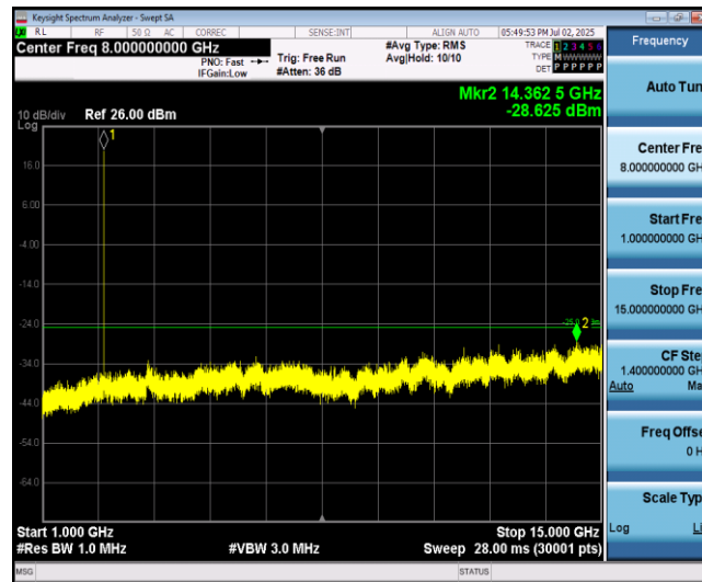
Band7-5MHz-16QAM-21100-1RB#0-Range2:1000~15000MHz
