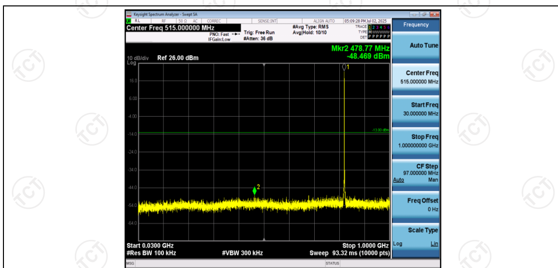
Band5-1.4MHz-QPSK-20407-1RB#0-Range1:30~1000MHz
