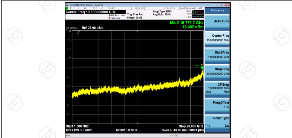
Band2-1.4MHz-QPSK-18607-1RB#0-Range2:1000~20000MHz
