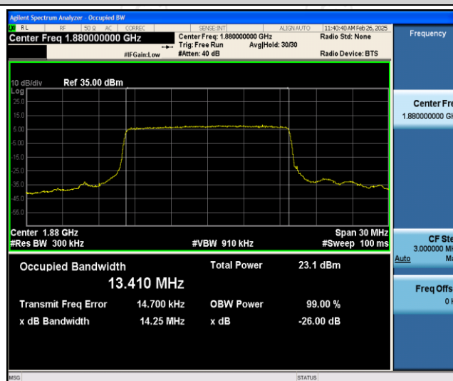
Band2-15MHz-QPSK-18900-75RB#0
