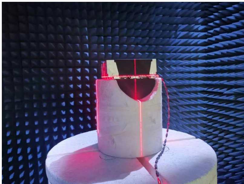
Free Space View of EUT
